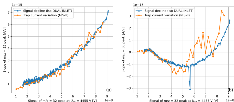
Figure 4. Slopes of linear peak top fits as a function of the signal intensity, computed as shown in Fig. 3. Panel (a) presents the data for the m/z = 35 peak tops (4450 V to 4475 V) and panel (b) shows those for m/z = 36 (4420 V to 4470 V). The corresponding data were obtained from a series of acceleration voltage scans of pure-oxygen gases performed at different signal intensities. For one series, gas was admitted to the mass spectrometer using the NIS-II and the signal intensity was varied by altering the trap current (see Fig. 3). For the second series, pure-oxygen gas was filled into the reference bellow of the iso DUAL INLET and then acceleration voltage scans were performed while the signal intensity decreased due to the steady consumption of gas. For NIS-II (trap current variation) and iso DUAL INLET (pressure decline) measurements, gas was sourced from the cylinders SC 632349 and SC 540546, respectively.
