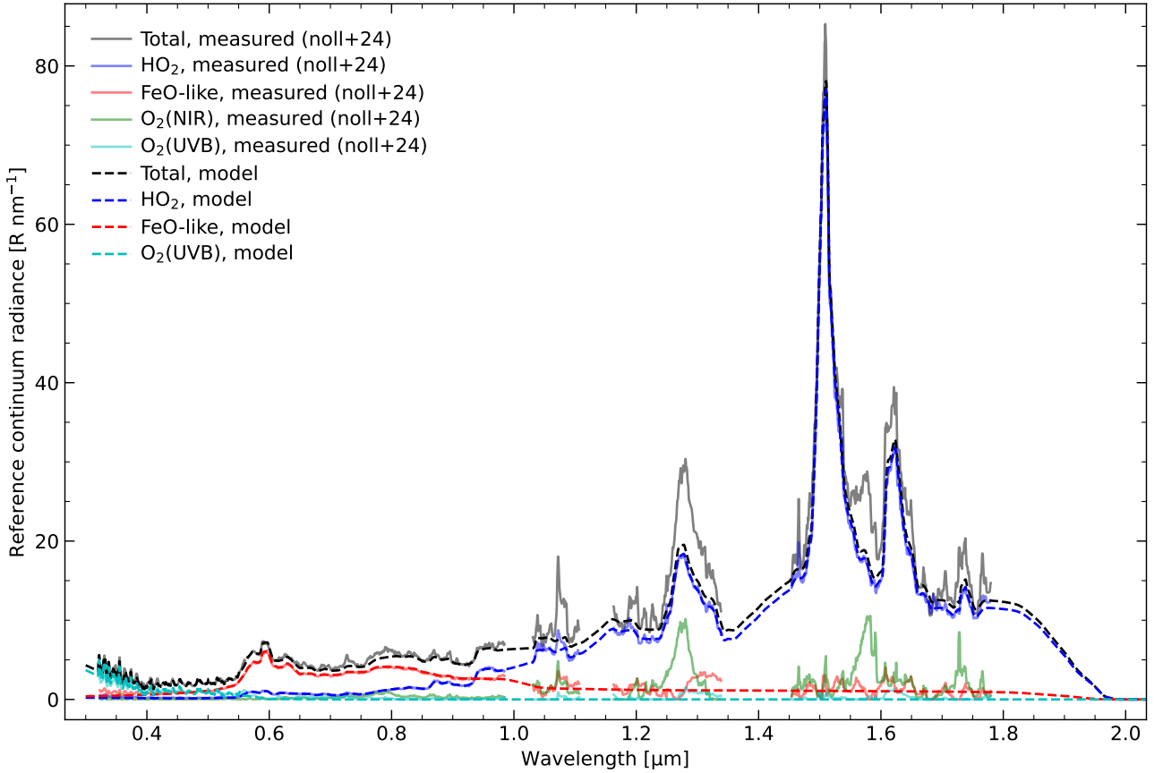
Figure 8. PALACE reference continuum model (dashed spectra) compared to X-shooter-based components from Noll et al. (2024a) (solid spectra with gaps). The total (black), \text{HO}_2 (blue), FeO-like (red), and \text{O}_2(\text{UVB}) emissions (cyan) are shown in both cases. The \text{O}_2(\text{NIR}) residuals (green) are not part of PALACE as they should be covered by the line emission model.
