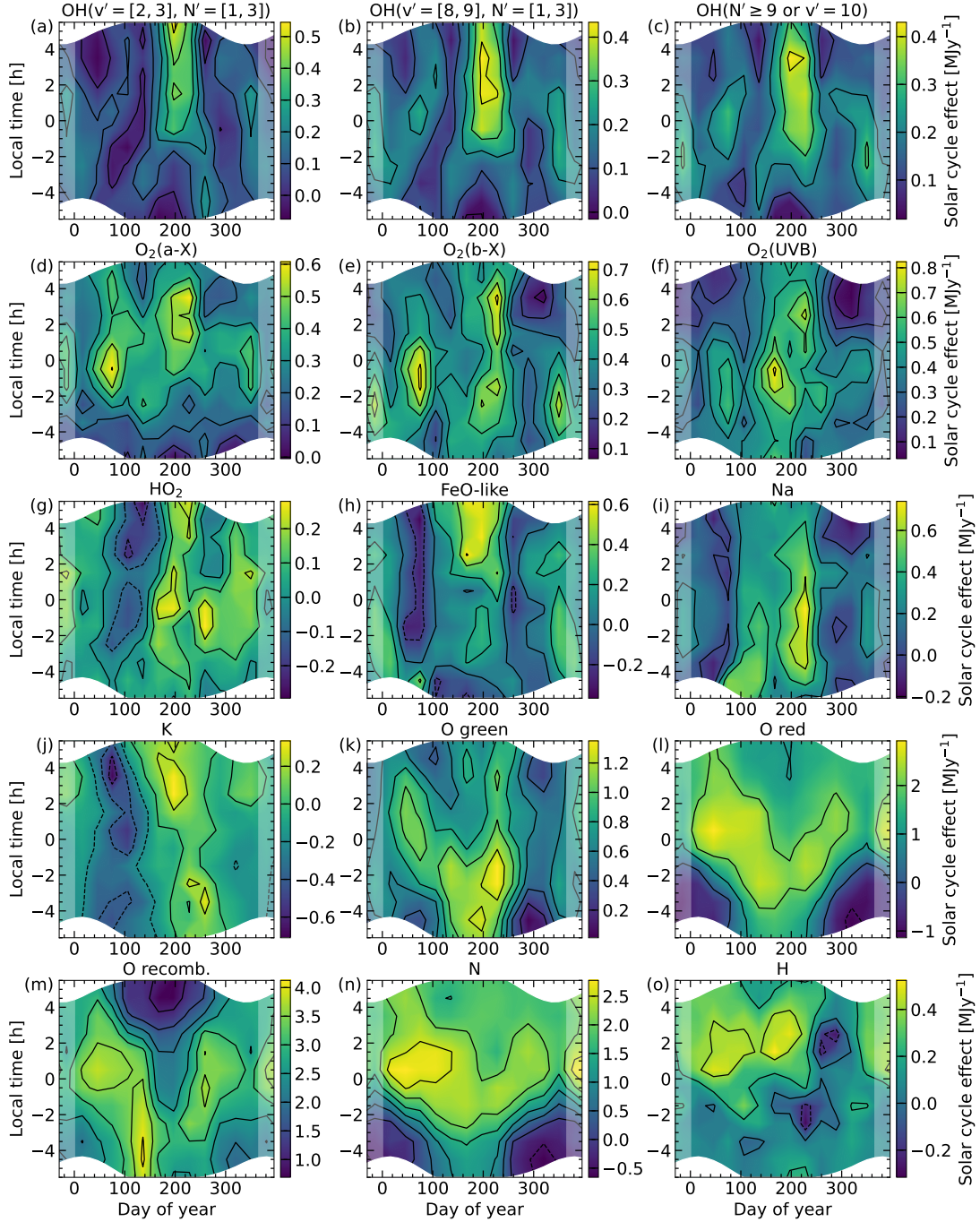
Figure 10. Climatologies of the relative intensity change by an increase of the solar radio flux by 100sfu or 1 MJy, m_{\text{SCE}} , with respect to local time and day of year for 15 PALACE variability classes as defined in Table 4. The solar cycle effect is provided relative to the corresponding relative intensities f_0 in Fig. 9.
