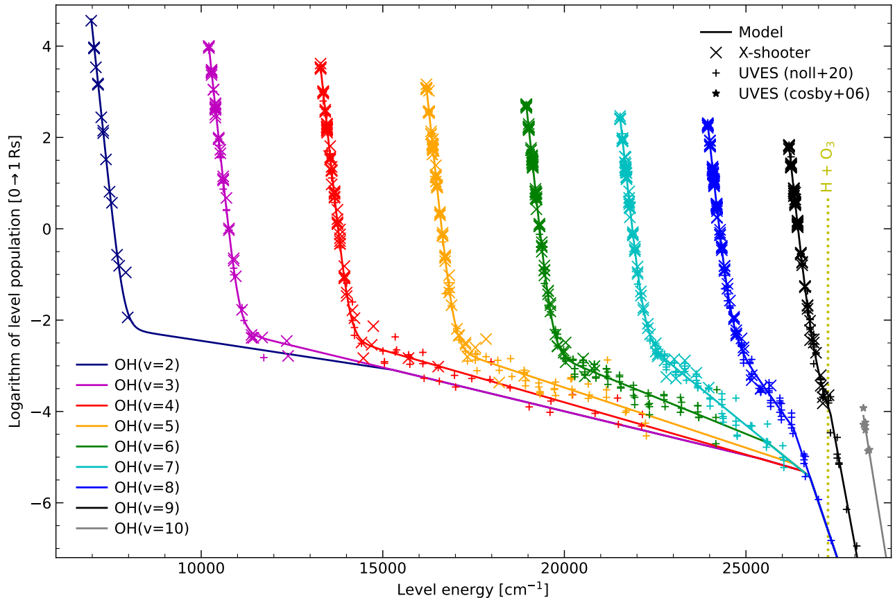
Figure 6. OH population model for the electronic ground state and vibrational levels v = 2 to 10 in logarithmic units and depending on the level energy. For v \leq 7 , 8 to 9 , and 10 , the model (solid lines) consists of two, three, and one fitted components, respectively. The corresponding parameters are provided in Table 3. The basic data for the v \leq 9 model originate from X-shooter measurements (crosses) and the UVES-related data from Noll et al. (2020) (plus signs). For v = 10 , UVES-based data from Cosby et al. (2006) (stars) were used. The energy provided by the OH-producing reaction of H and O 3 is marked by a vertical dotted line.
