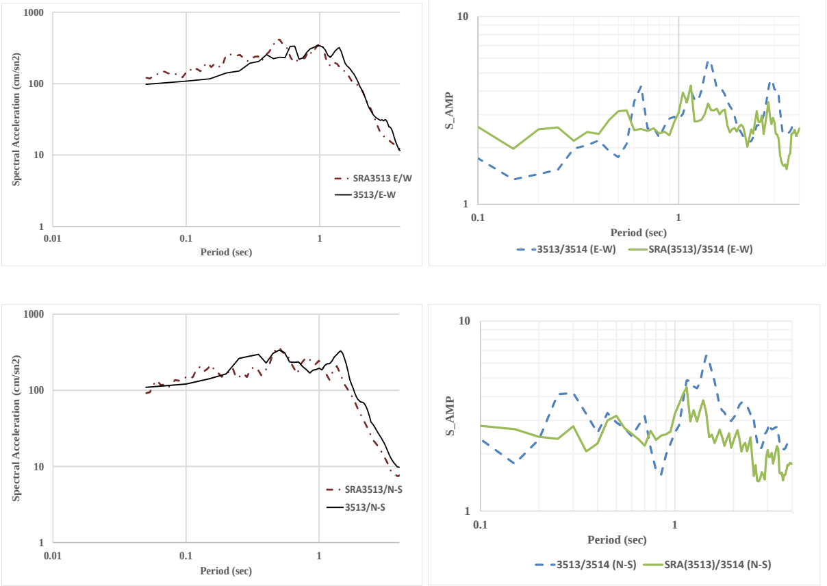
Figure 7. The comparison of recorded and estimated (SRA) elastic response and amplification spectra for 2020 Samos event@station 3513
