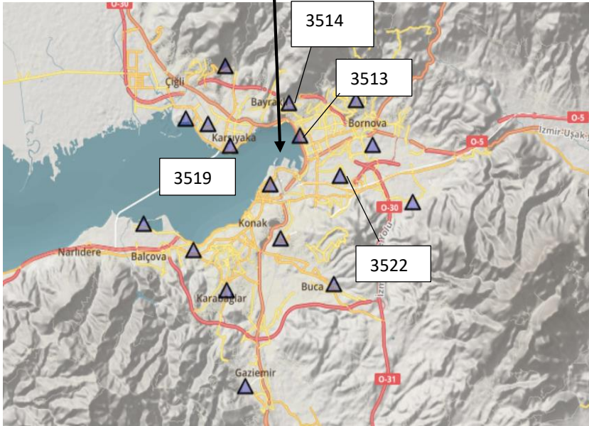
Figure 5. Overview of Stations in Izmir. (Base map adapted from AFAD TADAS ( https://tadas.afad.gov.tr ).)
