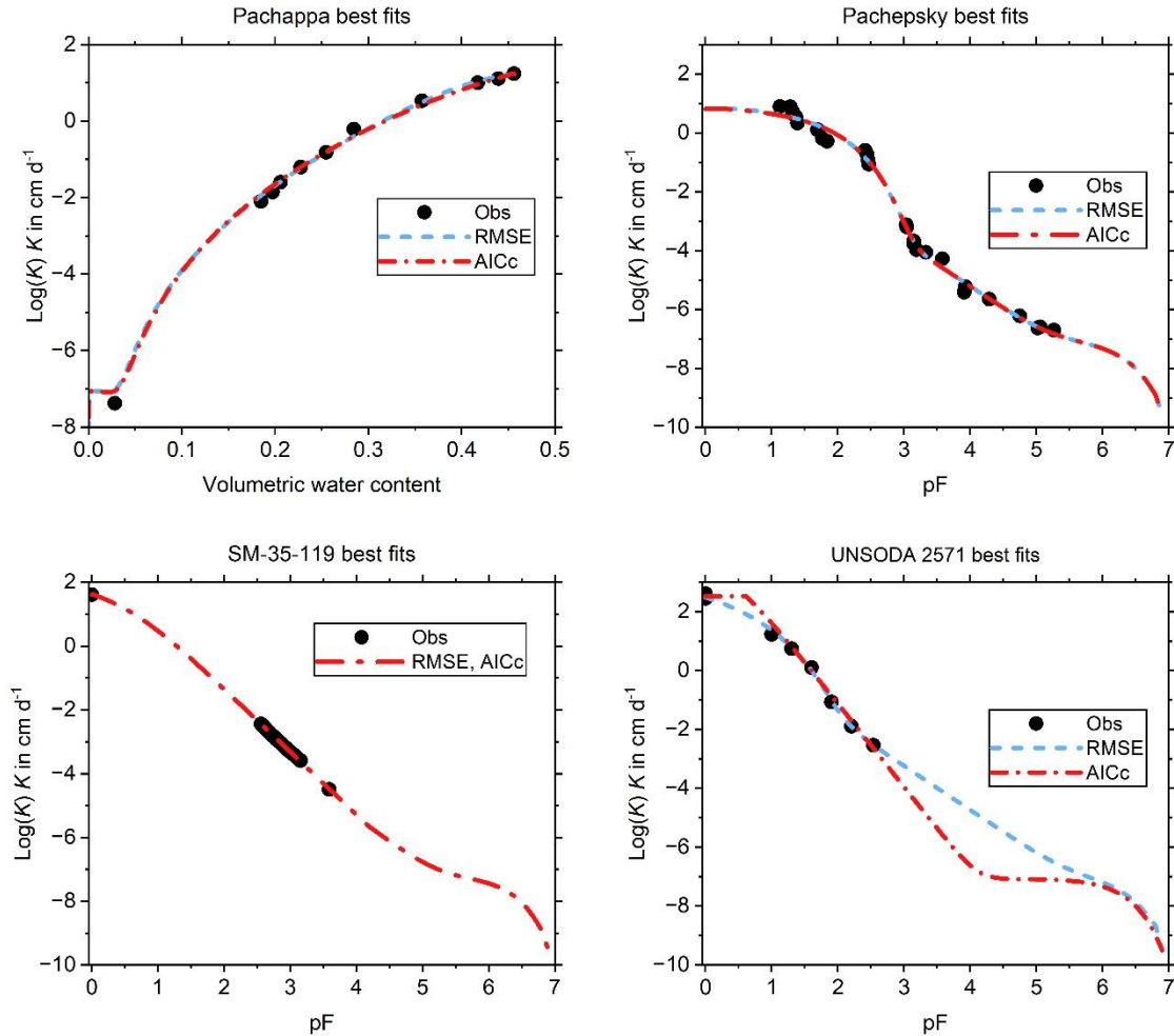
535 Figure 1: The fits that had either the smallest value of the Root Mean Square Error (RMSE) or Akaike's Information Criterion corrected for small samples (AICc) of all fits, i.e. those fits that are identified by the bold values in Tables 4–7. For Pachappa, the best performing UHCC models were ADV (RMSE) and JUV (AICc), for Pachepsky ADV (both RMSE and AICc), for SM-35-119 JUV (both RMSE and AICc), and for UNSODA 2571 ADV (RMSE) and JUV (AICc).
