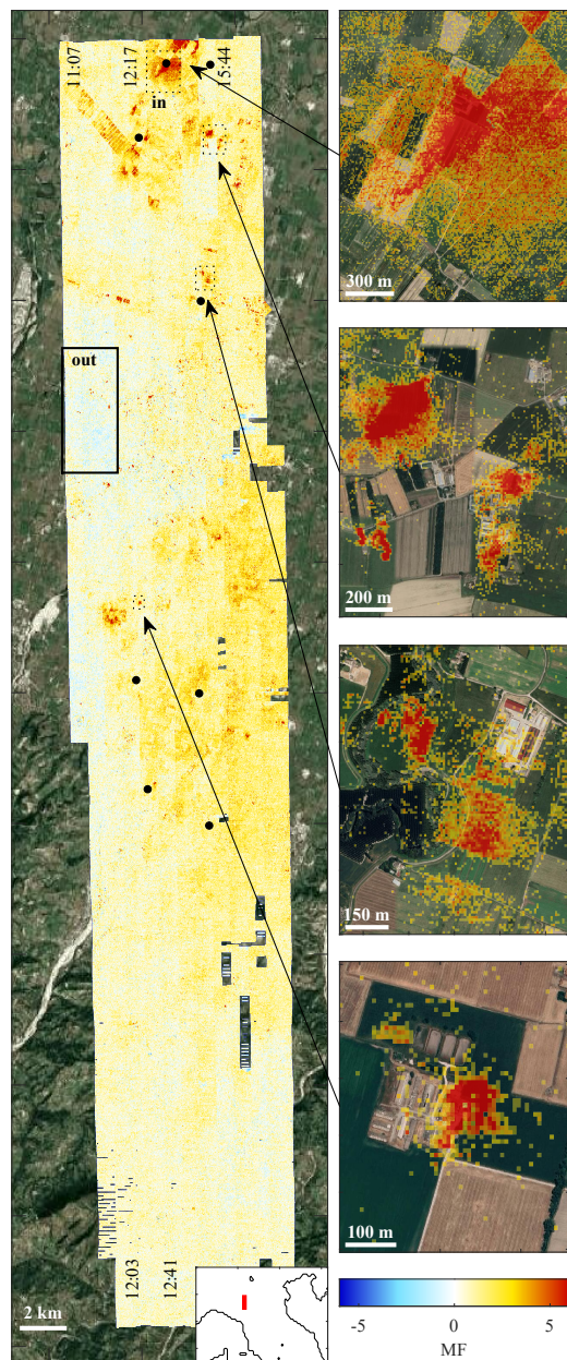
Figure 8. Superimposed on satellite visible imagery from © Google Maps, MF distribution retrieved from Hyper-Cam measurements performed over the Po valley (the location within Italy is shown in red in the inset) on 30 June 2022, revealing \text{NH}_3 hotspots over various farms. Some of these identified sources, delimited by dotted rectangles, are displayed on the right side of the figure. The black dots refer to the agricultural sources reported in the E-PRTR between 2020 and 2022. The local overflight time is indicated at the beginning of some flight tracks . The "in" and "out" boxes correspond to the areas used to estimate the SNR and FAR, and to renormalize MF.
