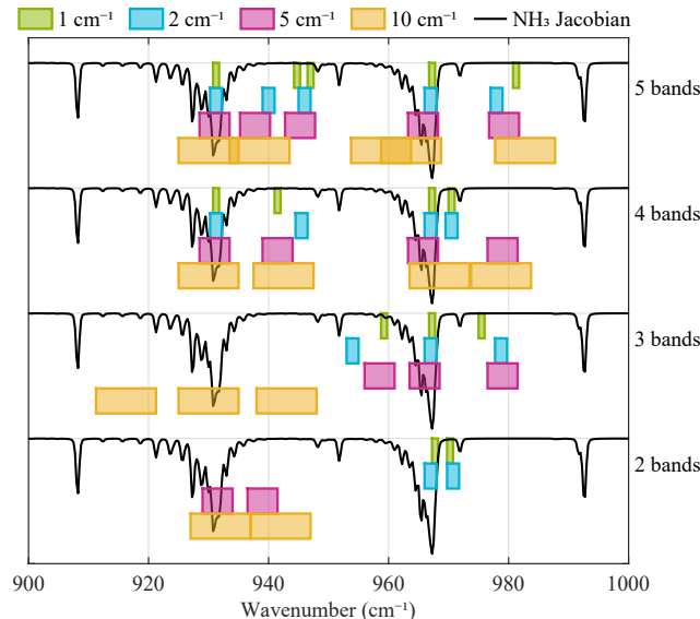
Figure 6. Illustration of the optimal spectral bands of various widths (from 1 to 10 cm -1 ) for observing atmospheric NH 3 in the infrared. The NH 3 Jacobian from Figure 1 is indicated as well in each subpanel (black line). Exact band positions are listed in Table 3.
