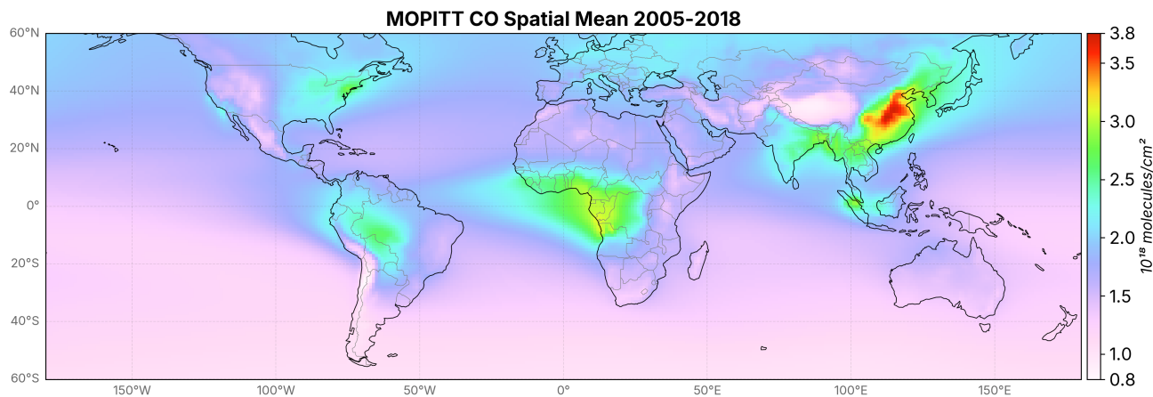
Figure 2. Temporally averaged global map of de-trended MOPITT CO over the period of 2005-2018 across the globe from 60°S to 60°N (in molecules \text{cm}^{-2} ).
