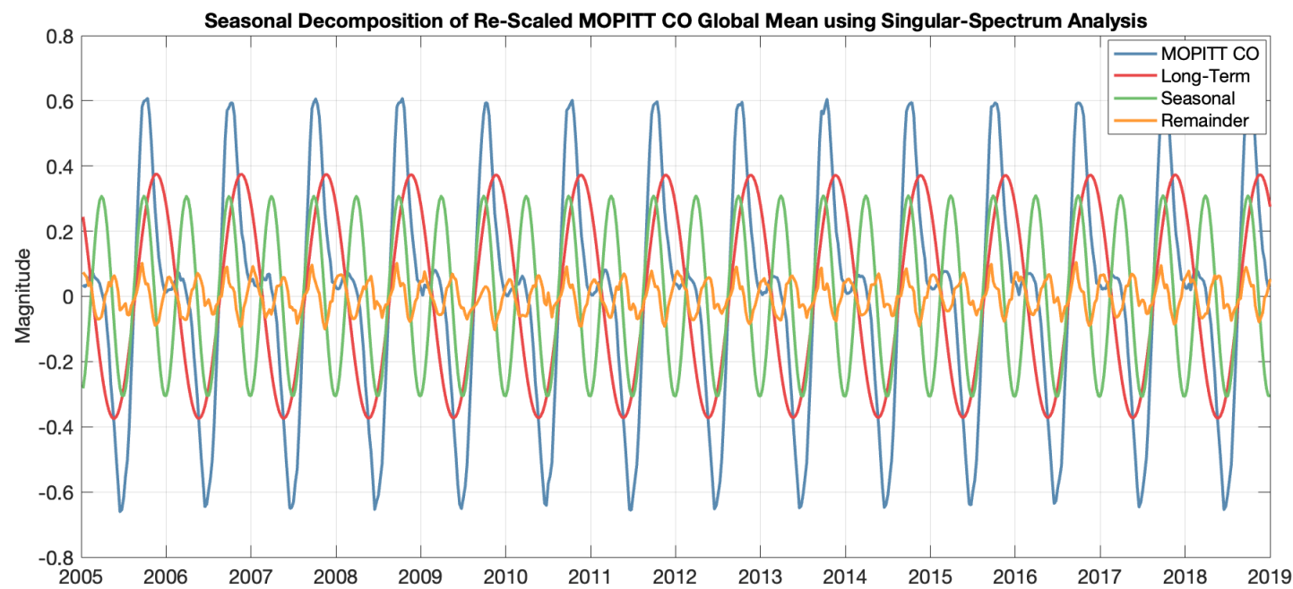
Figure 5. A time series plot of the spatially averaged MOPITT CO global mean (blue) and the long-term (red), seasonal (green) and remainder (orange) components of the SSA decomposition.
