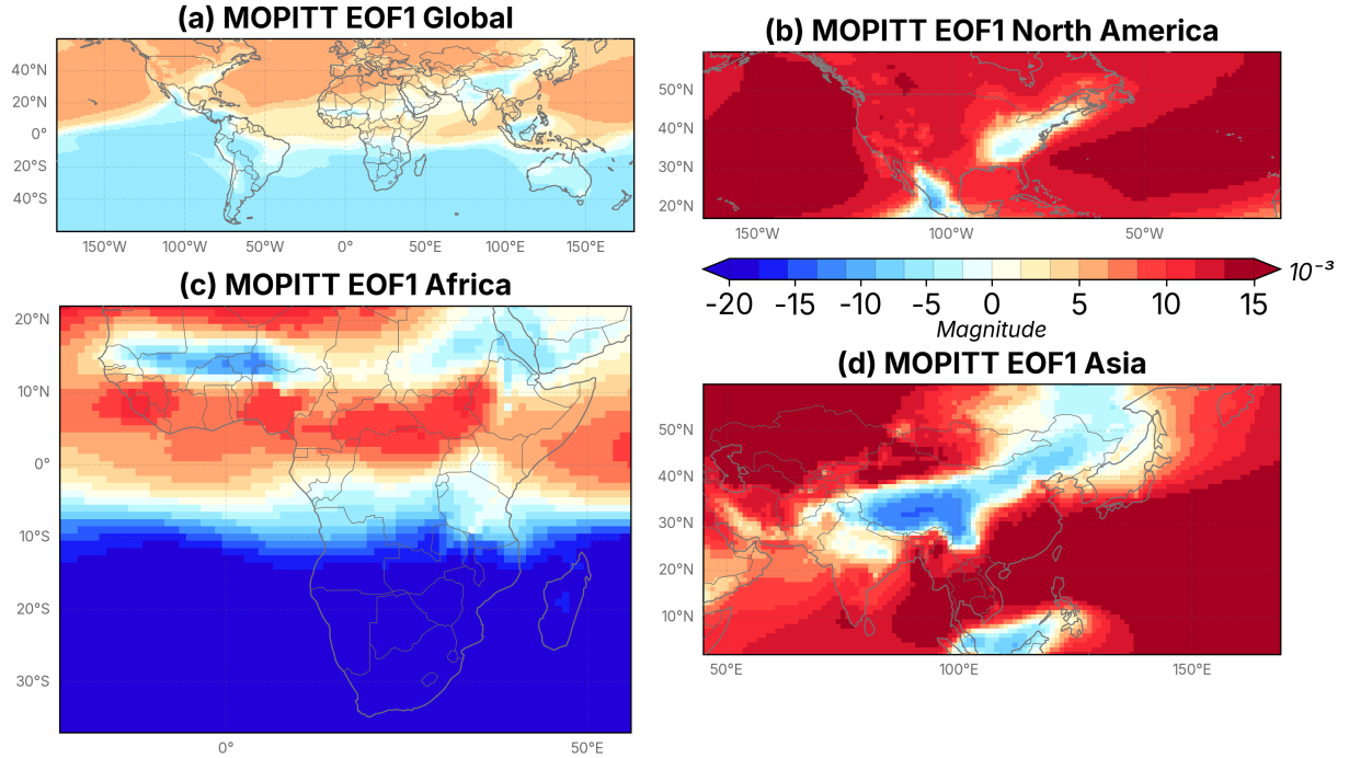
Figure 3. Spatial map showing the first EOF mode of MOPITT CO for (a) the globe, (b) North America, (c) Africa, and (d) Asia. All magnitudes are unitless, and all modes represented have unit norm.
