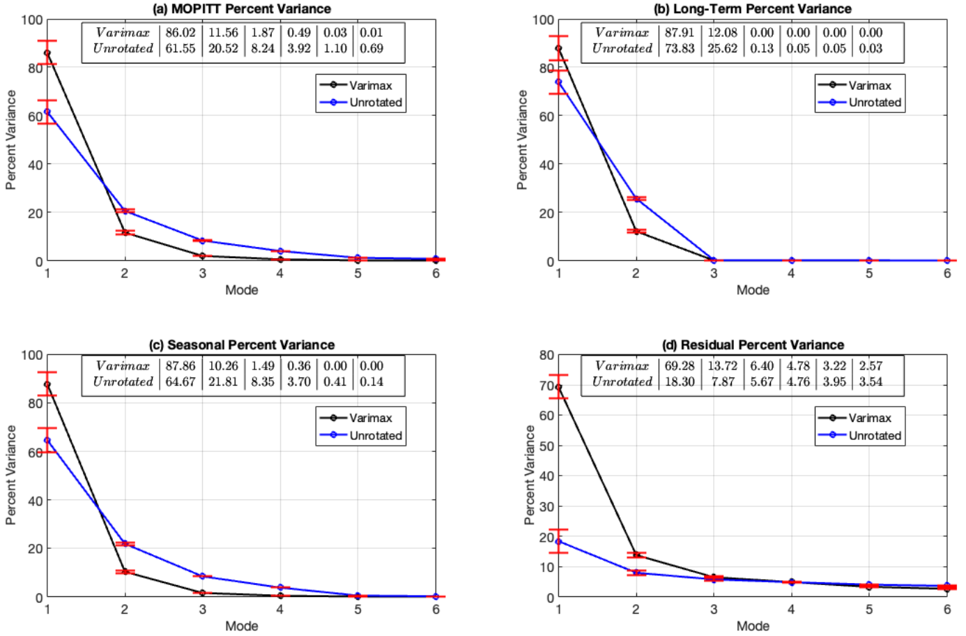
Figure 4. The percent variance that is explained by the first six normalized EOF modes for (a) the MOPITT dataset and (b) long-term, (c) seasonal, and (d) residual components after using an SSA decomposition. Results are shown globally for both varimax EOFs (black) and unrotated EOFs (blue). Our error bars computed using the North test are shown in red.
