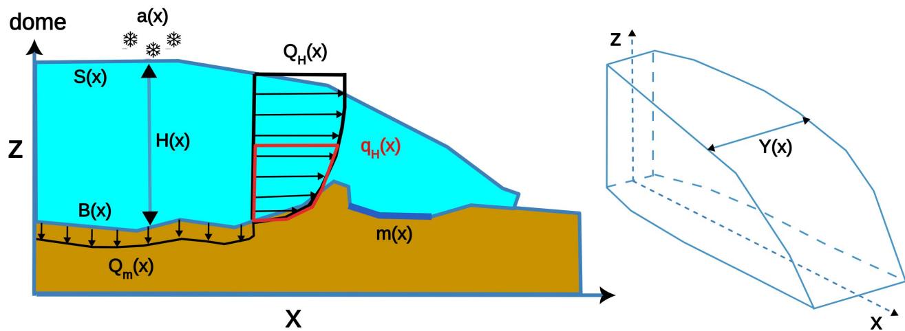
Figure 1: Diagram of the flow tube of an ice sheet with the principle notations used in this article.
