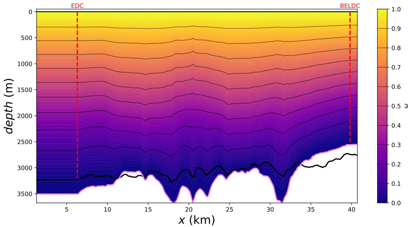
500 Figure 6: The \omega horizontal flux shape function along the DC-BELDC flow line. The positions of the EDC and BELDC deep drill sites are plotted in dashed red. The observed bedrock is in thick black and the mechanical bedrock ( the elevation where the extrapolated velocity becomes zero ) in violet. This figure was automatically generated by the age_flow_line-1.0 software.
