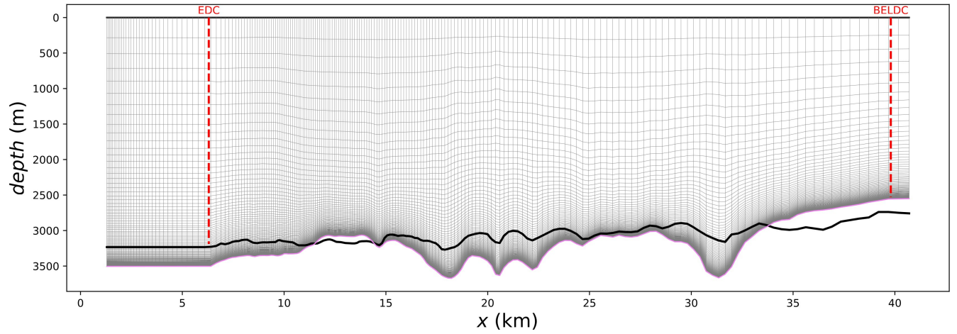
Figure 5: Mesh of the age_flow_line-1.0 model experiment in the (\pi, \theta) ( top ) and (x, z) ( bottom ) coordinate system. The positions of the EDC and BELDC deep drill sites are plotted in dashed red. The observed bedrock is in thick black and the mechanical bedrock in violet. For better readability, the resolution of the grids has been decreased by a factor of 5. Note that in the top panel, the EDC and BELDC ice cores do not extend down to the bottom of the mesh, since this mesh converges asymptotically towards the mechanical bedrock but never reaches it. These figures were automatically generated by the age_flow_line-1.0 software.
