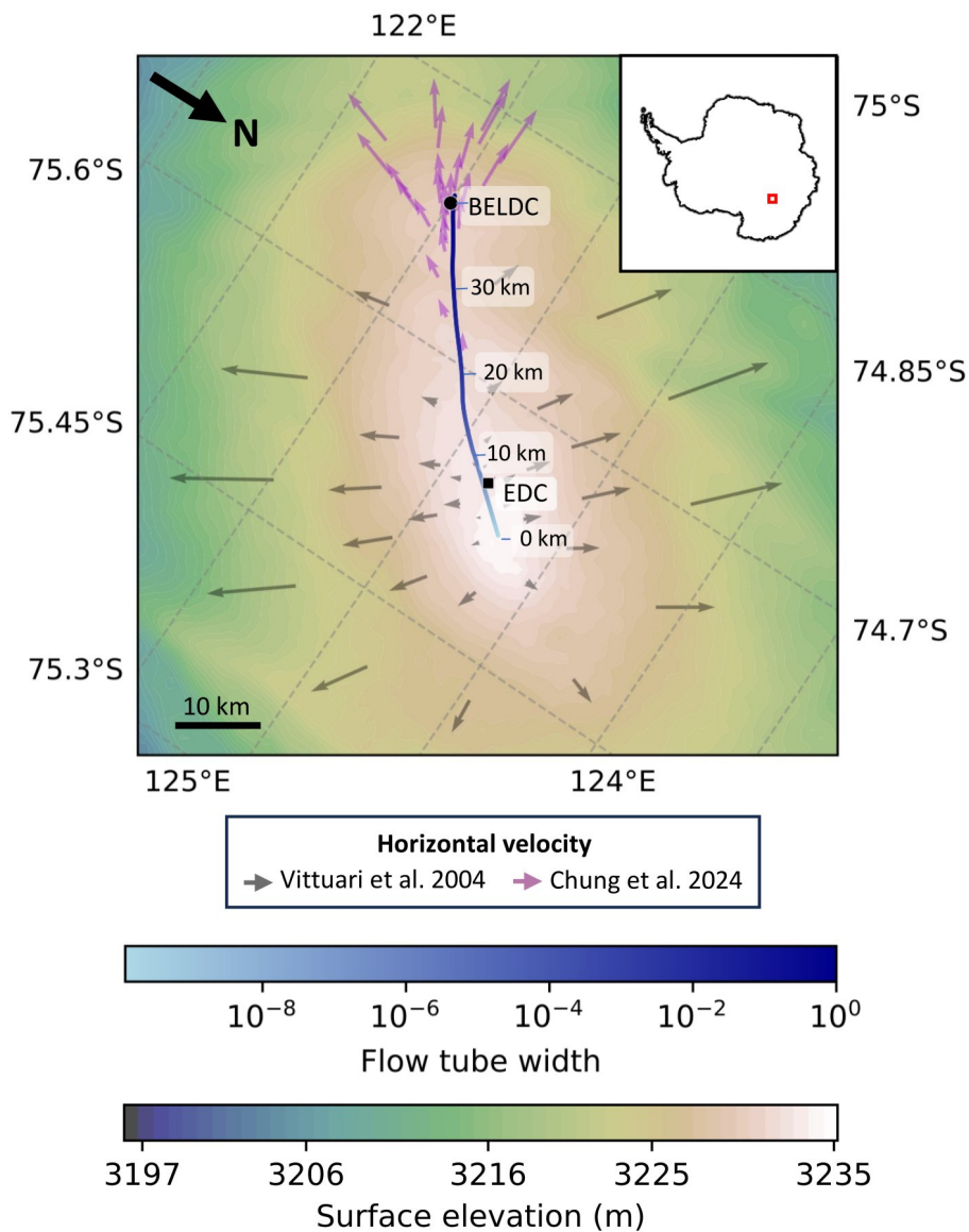
Figure 3: Map of the flow line (central blue line) going from DC to BELDC with the width of the flow tube according to the blue colour bar. Two pairs of adjacent flow lines ending at BELDC and 20 km downstream from the dome are also shown to emphasize the strong lateral flow divergence along this divide. The background colour represents the surface elevation. The grey and pink arrows represent surface velocity measurements. The dark red line represents the radar transect where the 1D inverse model of Chung et al. (2023) was applied. Adapted from Chung et al. (2024).
