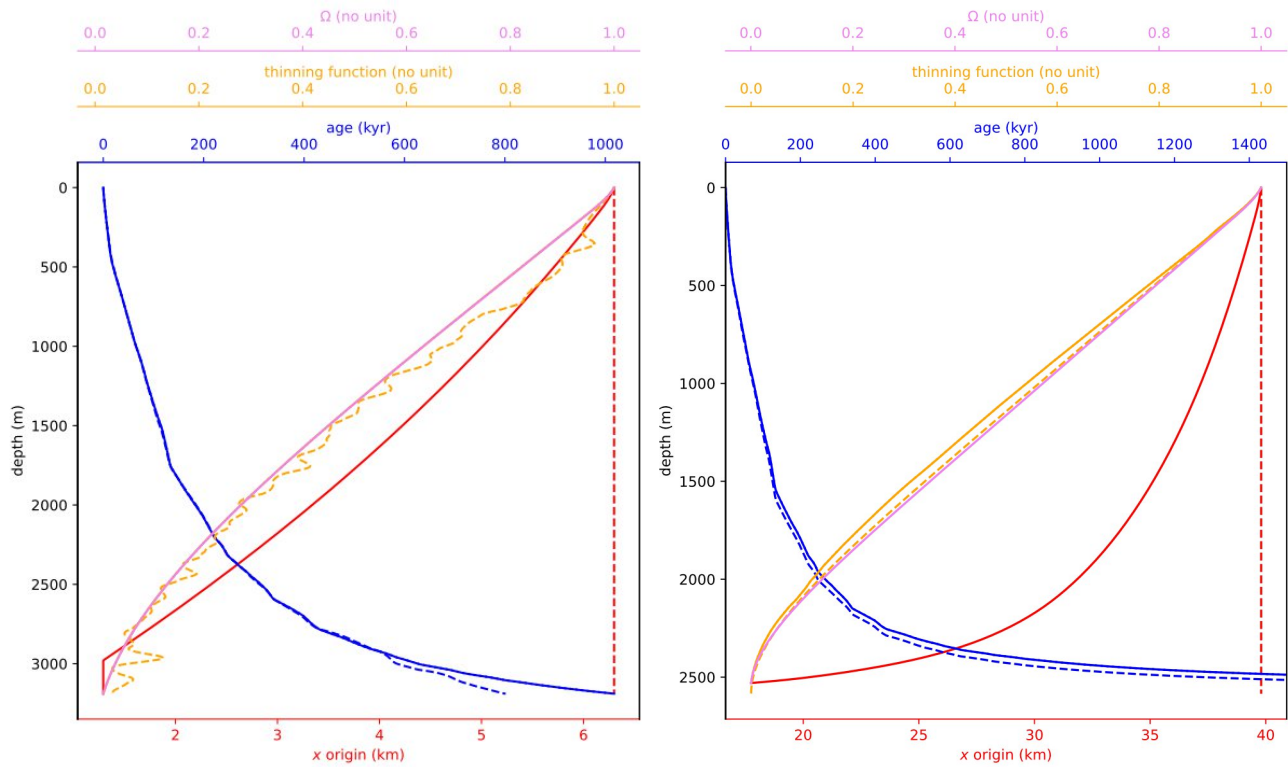
Figure 10: Age (blue), vertical thinning function (green/orange), \Omega flux shape function (violet) and spatial origin (red) of the ice at the EDC (left) and BELDC (right) drill site locations. The solid lines represent the 2.5D age_flow_line-1.0 results. The dashed lines represent the AICC2012 chronology for EDC and the results of the 1D model (Chung et al., 2023) for BELDC. Note that for EDC, the orange and violet solid lines are superimposed. These figures were automatically generated by the age_flow_line-1.0 software.
