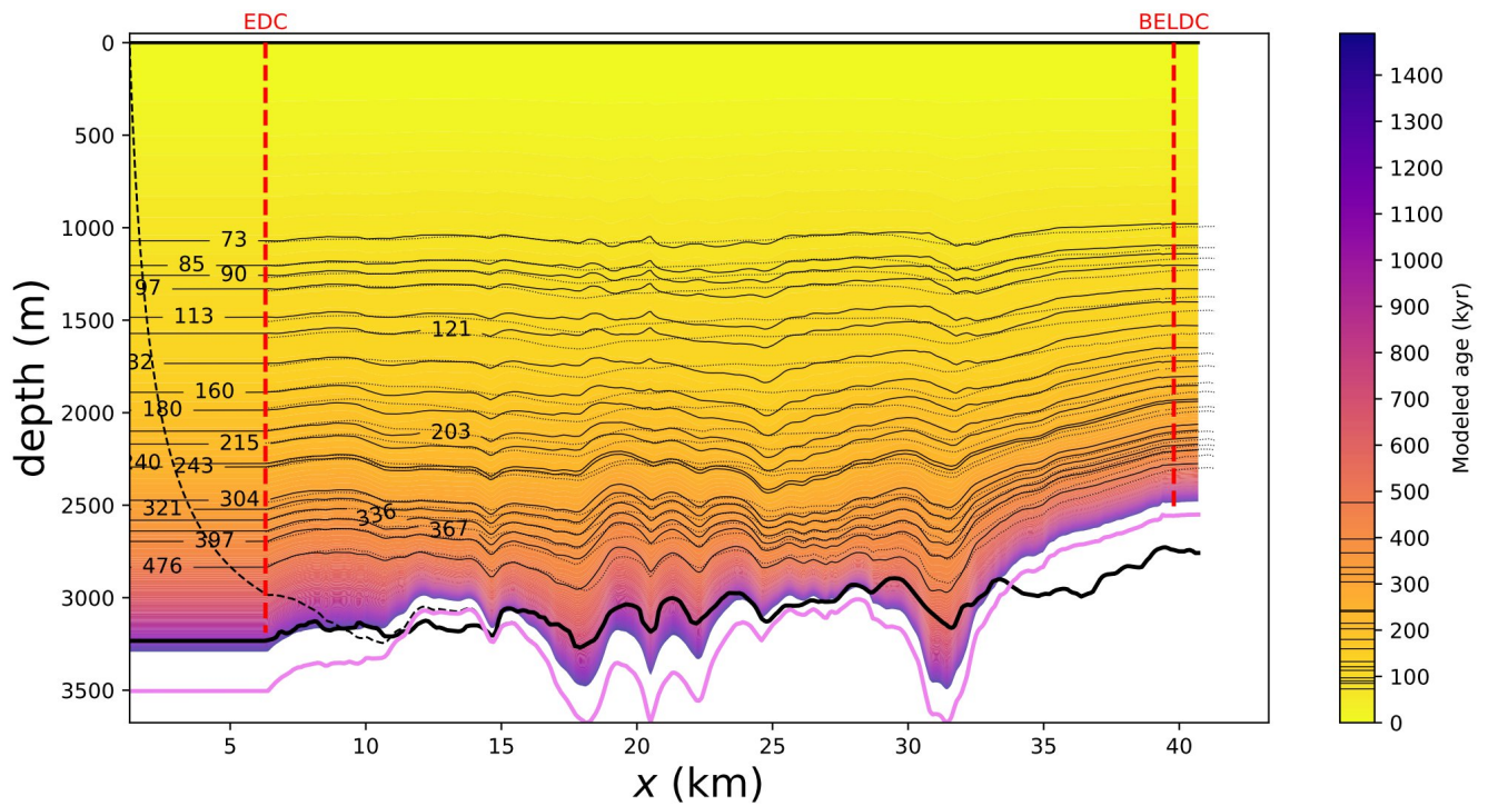
505 Figure 7: Modelled age along the DC-BELDC flow line, according to the colour scale on the right. The modelled isochrones are plotted in solid black and their age is represented on the colour bar. The positions of the EDC and BELDC deep drill sites are plotted in dashed red. The black dashed line represents the trajectory originating from the surface upstream corner. The dotted black lines are the isochrones observed by radar. The observed bedrock is in thick black and the mechanical bedrock in violet. This figure was automatically generated by the age_flow_line-1.0 software.
