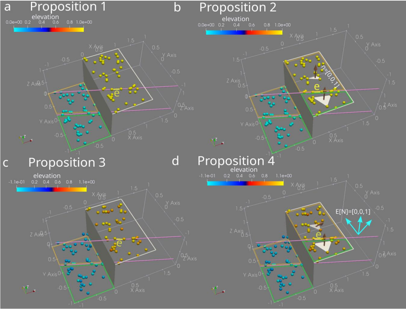
165 Figure 3 Workflow in the theoretical part of the study (a) this panel relates to Proposition 1. In this proposition, an edge e is fixed on the surface of the footwall. Then, the dip directions of triangles depend on whether the third point sampled from the hanging wall lies either to the left or right of e . The points on the surfaces of the hanging wall and footwall have constant elevation; (b) this panel relates to Proposition 2 and it shows a more general scenario than presented in the (a) panel. Here, for a fixed edge e , dip directions of triangles depend on whether the third point lies either to the left or right of e . We do not require from the points to lie on the hanging wall because the [0, 0, 1] vectors from the footwall will not affect the average dip direction of triangles. (c) Here, we add uncertainty to the elevation of points (Proposition 3). Then, for a fixed edge e , we investigate the average dip direction of triangles with the third point from the hanging wall. (d) the last 170
