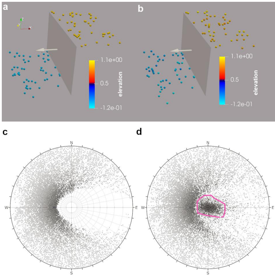
Figure 5 A geological horizon displaced by a vertical fault; its normal vector points to the West (azimuth 270°) (a) a case study with elevation data without errors; (b) a case study with points having elevation data with errors (mean=0, standard deviation=0.05), (c) a spherical projection for the orientation measurements as three-element subsets ( n=122304 ) of the points corresponding to panel (a) (d) a spherical projection for the orientation measurements as three-element subsets ( n=161700 ) of the points corresponding to panel (b). The small cloud at the centre of the plot (pink polygon) corresponds to almost flat triangles lying entirely on the same side of the fault. The spherical projection was conducted using Dips software (Rocscience, 2017). We used pole vectors, upper hemisphere and equal angle projection.
