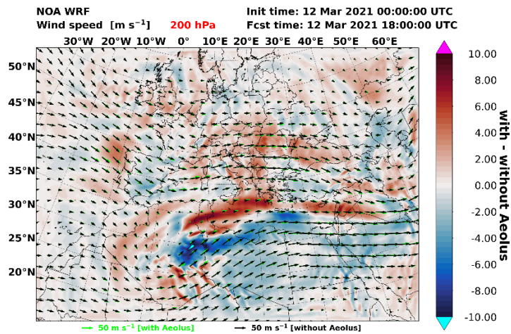
Figure A 4: Wind speed (m/s) in WRF 18 h forecasts. Horizontal winds (a) “w” Aeolus assimilation, (b) “w/o” Aeolus assimilation and (c) wind speed differences (“w” – “w/o” Aeolus assimilation) at 200 hPa (~12 km).
