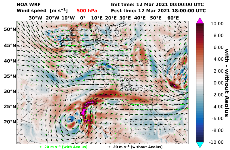
Figure A 5: Wind speed (m/s) in WRF 18 h forecasts. Horizontal winds (a) “w” Aeolus assimilation, (b) “w/o” Aeolus assimilation and (c) wind speed differences (“w” – “w/o” Aeolus assimilation) at 500 hPa (~5.5 km).
