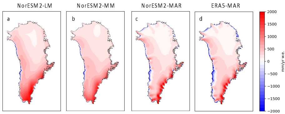
Figure S1 Similar to Figure 5 but including results for NorESM2-LM-EC with 2° horizontal resolution of the atmosphere model. Mean surface mass balance over the period 1960-1989 from a) low-resolution NorESM2-LM-EC, b) NorESM2-MM-EC, c) NorESM2-MAR and d) ERA5-MAR). All fields are masked to the modelled ice sheet area in NorESM2 at the end of year 2014.
