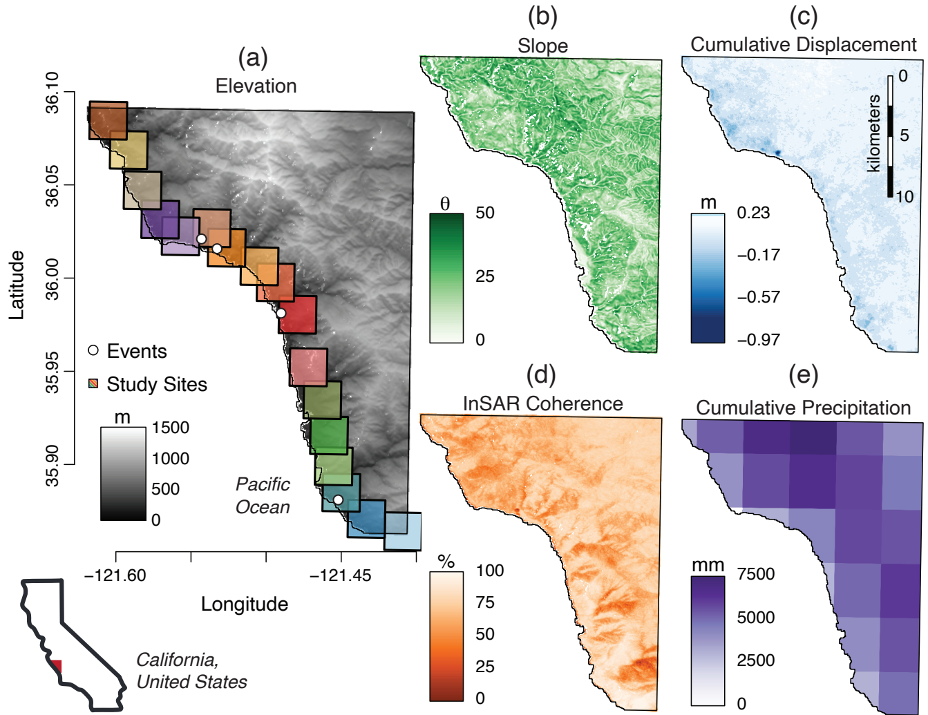
Figure 1. Regional scale maps of study area. (a) Digital elevation model of the study area. The 4 recorded landslide events by USGS and CA are shown as white dots. The black outlined boxes are the 17 sub-regions we used in this analysis. (b) Topographic slope angle (degrees). (c) Cumulative displacement from Sentinel-1 InSAR from Nov 2015 to Dec 2022. (d) InSAR temporal coherence map. (e) Accumulated precipitation from PRISM from 1 Nov 2015 to 30 Nov 2022.
