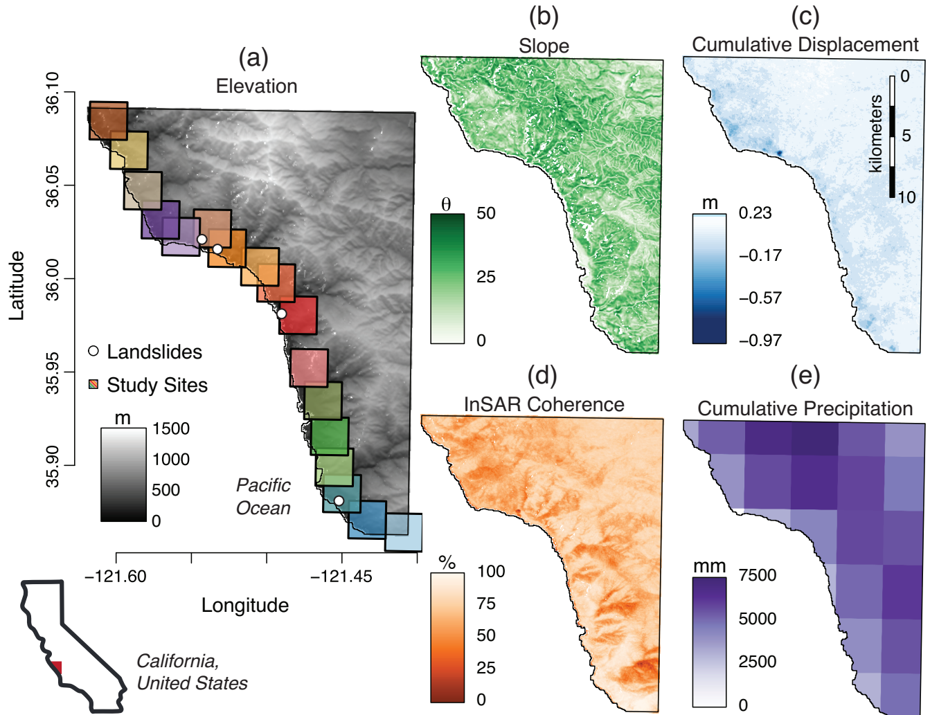
Figure 1. Regional scale maps of study area. (a) Digital elevation model of the study area. The 4 recorded landslide events landslides by USGS and CA are shown as white dots. The black outlined boxes are the 17 sub-regions we used in this analysis. (b) Topographic slope angle (degrees). (c) Cumulative displacement from Sentinel-1 InSAR from Nov 2015 to Dec 2022. (d) InSAR temporal coherence map. (e) Accumulated precipitation from PRISM from 1 Nov 2015 to 30 Nov 2022.
