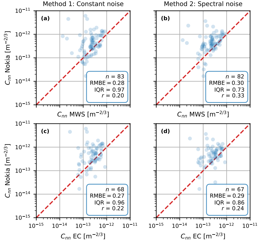
Figure 9. 30-min C_{nn} estimates obtained with the Nokia CML for all time intervals in the validation part of our data, post-processed with the constant-noise method (a and c) and spectral-noise method (b and d) versus the MWS (a and b) and the EC (c and d) estimates, corrected for the height difference (Sect. 3.3). The red line is the 1:1 line. For the calibration results, see Fig. E1.
