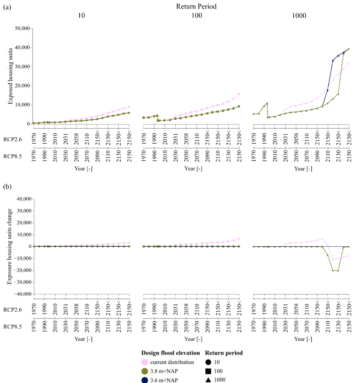
435 Figure 7: Influence of design flood elevation on the number of exposed houses. The top three figures show the absolute number of exposed houses when the current elevation distribution per neighborhoods is applied for new housing units, design flood elevation NAP +3.8 m gives the situation when building lots are raised to NAP +3.8 m. The lower three figures are relative to the reference.
