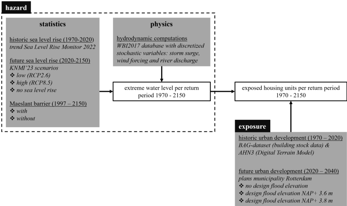
165 Figure 2: Schematic of the integrated methodological framework and data inputs for calculating residential flood exposure. This diagram shows how flood hazard inputs (derived from sea level statistics, hydrodynamic models, and Maeslant storm surge barrier scenarios) are combined with exposure inputs (historical building stock, future urban development plans, and design elevation scenarios) to determine the number of exposed housing units per return period from 1970 to 2150.
