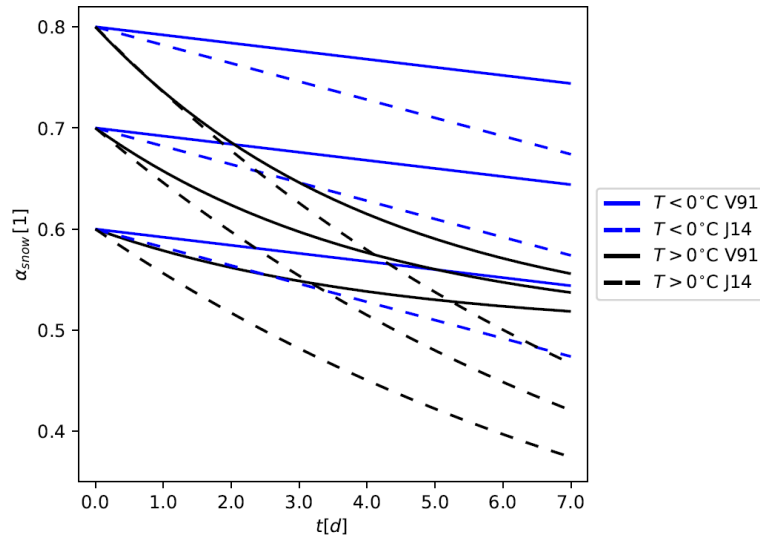
Figure 2. Linear (blue) and exponential (black) decrease of albedo of snow pack \alpha_{\text{snow}} (Eqs. 35-36) as applied in METRAS ( \alpha_{\text{min}} = 0.5 , \tau_{T,\alpha} = 0.24 , \Delta t = 5\text{s} ) after Versegny (1991) (V91, solid lines) and as applied in MITRAS ( \alpha_{\text{min}} = 0.18 , \tau_{T,\alpha} = 0.11 , \Delta t = 0.1\text{s} ) after Järvi et al. (2014) (J14, dashed lines).
