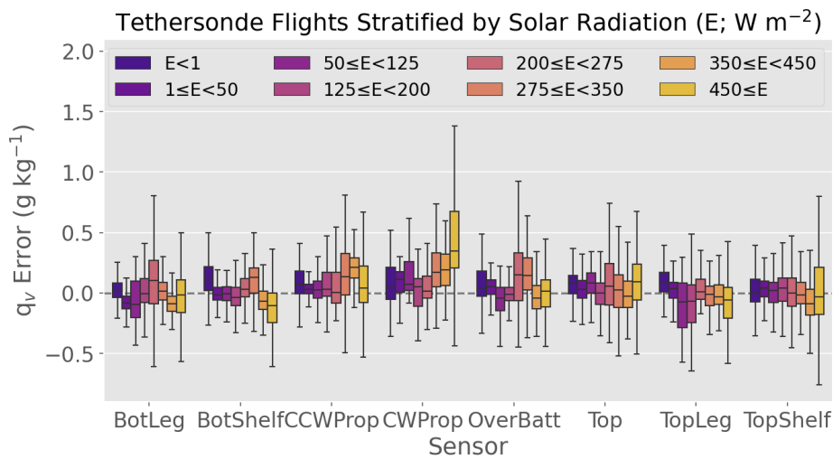
455 Figure 7: As in Figure 4, but for water vapor mixing ratio errors.
