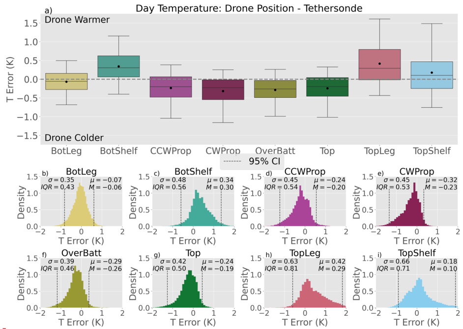
295 Figure 3: (a) Box plots of the drone sensor temperature minus the tethersonde sensor temperature, i.e. the “errors” (positive values indicate that the drone is warmer than the tethersonde), for all daytime flights. The box outlines denote the 25th, 50th, and 75th percentiles, whiskers extend to the 5th and 95th percentiles, and the dots indicate the distribution means. (b-i) Density histograms of the daytime flight temperature errors for each individual drone sensor as labeled on each panel. The 2.5th and 97.5th percentiles are marked with dashed vertical black lines to indicate the 95% confidence interval. The error standard deviation ( \sigma ), mean ( \mu ) , 300 median (M) , and interquartile range (IQR) of the error are labeled at the top of each panel.
