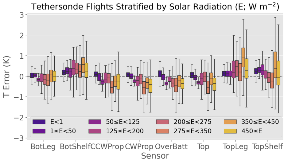
Figure 4: As in Figure 3a, except that for each sensor position, the tethersonde data is stratified by solar radiation, E ( \text{W m}^{-2} ), observed by the surface weather station.
