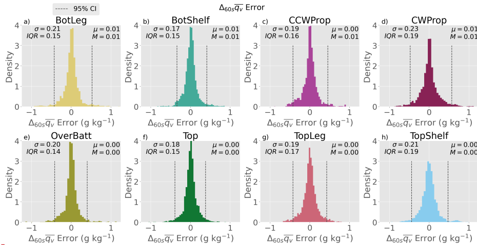
Figure 10: As in Figure 8, but for \Delta_{60s} \bar{q}_v , where \bar{q}_v is water vapor mixing ratio.
