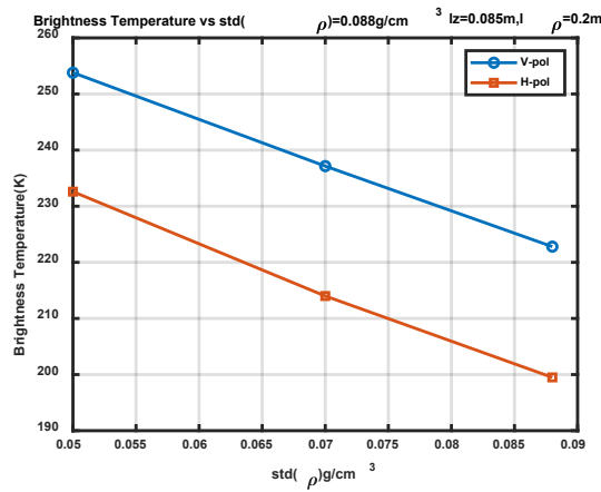
365 Figure 12 Brightness temperature changes with respect to std( \rho ) V-pol and H-pol both decrease as the value of std( \rho ) Increases.
