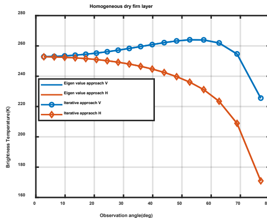
545 Figure A2: A single homogenous dry firm layer results from eigen value method and the iterative approach. The results from the two methods agree very well with each other.
