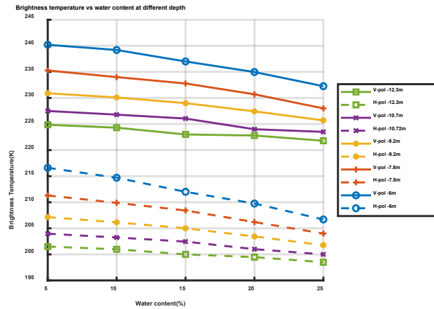
Figure 9 Brightness temperature as a function of liquid water content in the firm aquifer with the water table at different depths.
