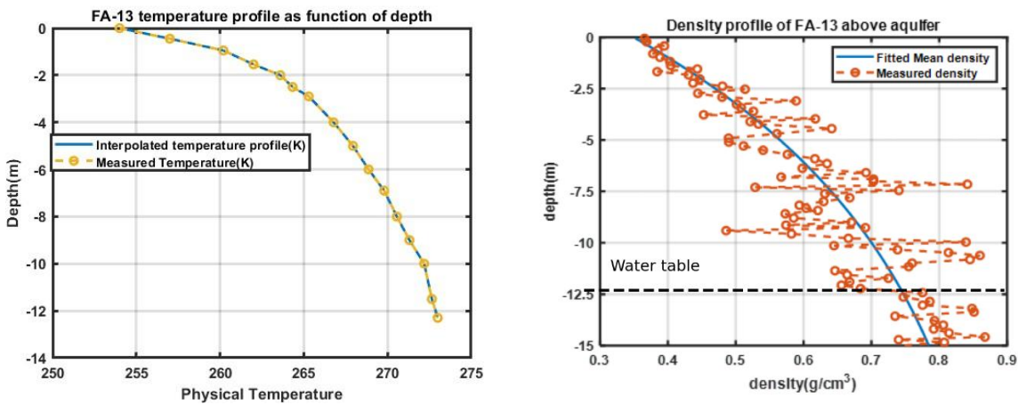
175 Figure 4 Temperature(left) and density profiles of FA13 from [Koenig et al. 2013, and Montgomery et al. 2018]. The measurements are taken on a scale of 0.5 meters.
