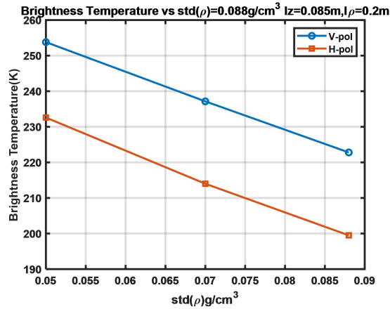
Figure 12 Brightness temperature change with respect to \text{std}(\rho) V-pol and H-pol both decrease as the value of \text{std}(\rho) Increases.
