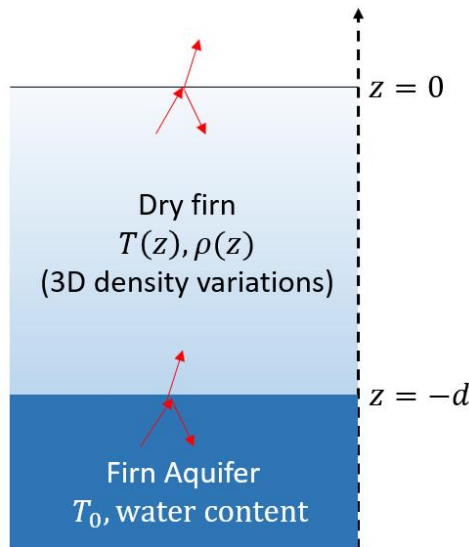
Figure 1 A two-layer model for the firn aquifer emission problem in the early spring before the surface melt starts. The top region is air( z > 0 ), middle region is dry firn with changing properties. The density fluctuation in this region is considered as 3 dimensional. The lower part is firn aquifer with a constant temperature of T_0 = 273.15 .
