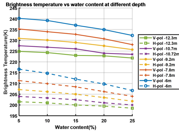
Figure 9 Brightness temperature as a function of liquid water content in firn aquifer with water table at different depths.
