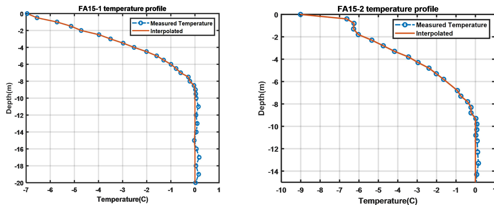
Figure C1 Temperature(left) of FA15-1 and FA15-2 [O.Miller et al. 2017]. The water table locations are -19.8m and -14.4m respectively. Unlike what is observed in FA-13, where the physical temperature becomes 0°C at the interface of the dry firn and aquifer, the physical temperature profiles in these two boreholes reach 0°C before reaching the aquifer water table
