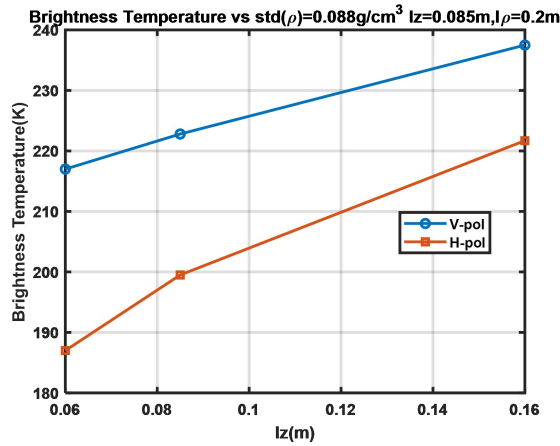
360 Figure 13 Brightness temperature changes with respect to l_z . With smaller l_z , the reduction to brightness temperature gets stronger.
