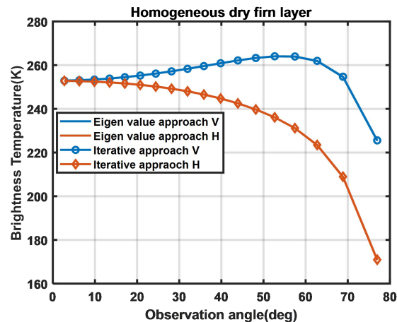
495 | Figure A2 , A single homogenous dry firn layer results from eigen value method and iterative approach. The results from the two methods agree very well with each other.
