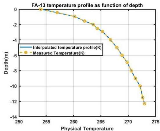
Figure 4 Temperature(left) and density profiles of FA13 from [Koenig et al. 2013, and Montgomery et al. 2018]. The measurements are taken on a scale of 0.5 meters.
