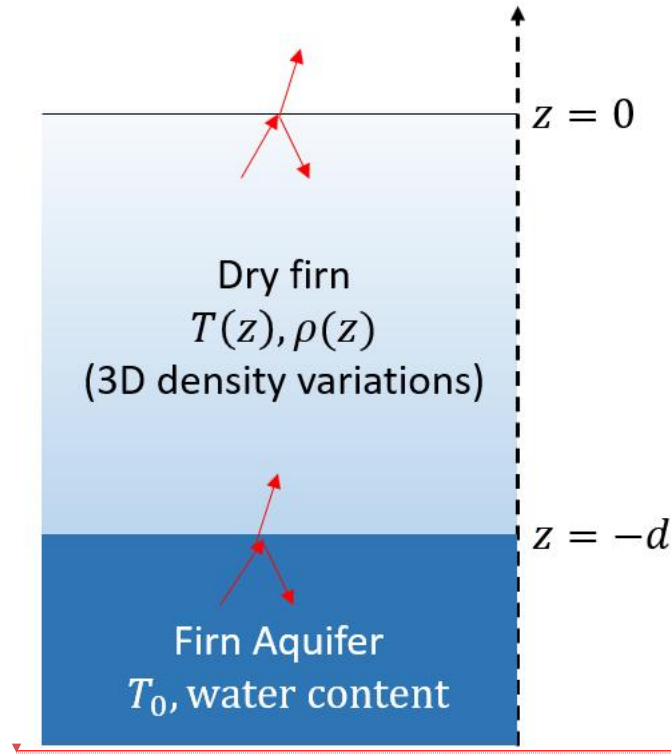
Figure 1 A two-layer model for the firn aquifer emission problem in the early spring before the surface melt starts. The top region is air ( z > 0 ), middle region is dry firn with changing properties. The density fluctuation in this region is considered as 3 dimensional. The lower part is firn aquifer with a constant temperature of T_0 = 273.15 .
