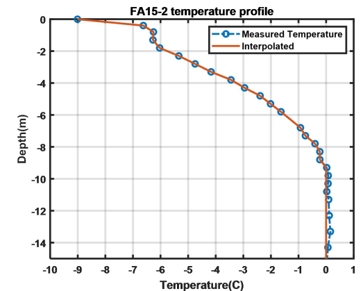
Figure 15 Temperature(left) of FA15-1 and FA15-2 [O.Miller et al. 2017]. The water table locations are -19.8m and -14.4m respectively. Unlike what is observed in FA-13, where the physical temperature becomes 0^{\circ}\text{C} at the interface of the dry firn and aquifer, the physical temperature profiles in these two boreholes reach 0^{\circ}\text{C} before reaching the aquifer water table
