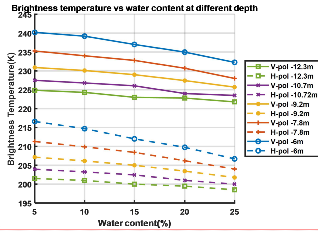
310 Figure 9 Brightness temperature as a function of liquid water content in firn aquifer with water table at different depths.
