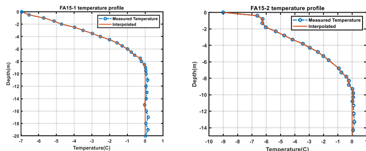
Figure 15: Temperature(left) of FA15-1 and FA15-2 [O.Miller et al. 2017]. The water table locations are -19.8m and -14.4m respectively. Unlike what is observed in FA-13, where the physical temperature becomes 0°C at the interface of the dry firm and aquifer, the physical temperature profiles in these two boreholes reach 0°C before reaching the aquifer water table
