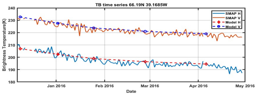
Figure 8 Time series forward modeling of Brightness temperature at location 66.19N 39.1685W. The mean density profile is obtained from FA-13. The physical temperature profile uses the FA-13 profile but is adjusted to have a slower changing speed according to depth. The water-table location is obtained by the GPR echogram by KU's Accumulation Radar.
