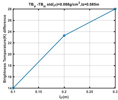
Figure 1415 The brightness temperature difference between V and H pol with respect to horizontal correlation length.
