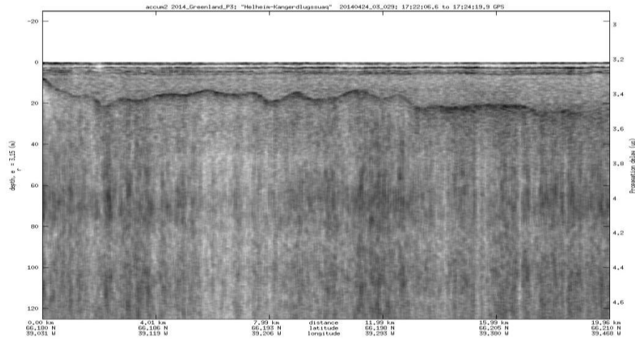
Figure 1819 Accumulation Radar data in 2014 near FA-13
