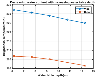
Figure 11 Figure 12 plots brightness temperatures for the cases when the liquid water content increases and decreases with respect to the water table depth. The left figure shows the case where liquid water content increases as water table depth decreases. The figure indicates that the decrease in water table depth, when accompanied by an increase in water content, results in a more pronounced reduction in brightness temperature than that caused by the decrease in water table depth alone. As can be observed from the figure, the increased water content contributes constructively to the decreased water table depth. The overall effect contributed to a 20K reduction in V-pol and an 18K reduction in H-pol. On the other hand, for the righthand side figure, the decreasing water content counters the effects of the increasing depth. The overall effects decrease the change of brightness temperature with respect to depth. The V-pol decreases by 7k, and the H-pol decreases by only about 5K in total. The parameters of std(\rho) , l_z and l_\rho are the parameters that control the properties of volume scattering in the dry firm.
