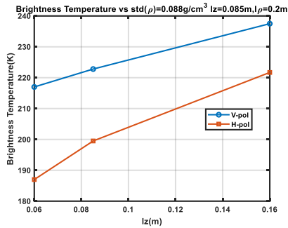
Figure 1314 Brightness temperature changes with respect to lz. With smaller lz, the reduction to brightness temperature gets stronger.
