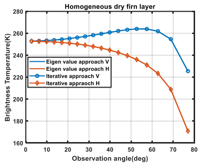
Figure 1748 A single homogenous dry firn layer results from eigen value method and iterative approach. The results from the two methods agree very well with each other.
