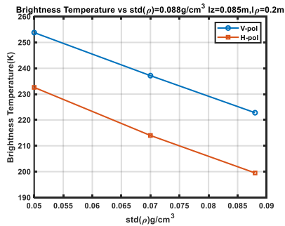
Figure 12 Brightness temperature change with respect to std(\rho) V-pol and H-pol both decrease as the value of std(\rho) Increases.
