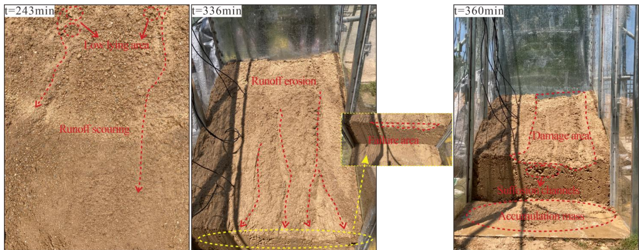
Figure 5. Deformation and failure process of the E1 slope.
