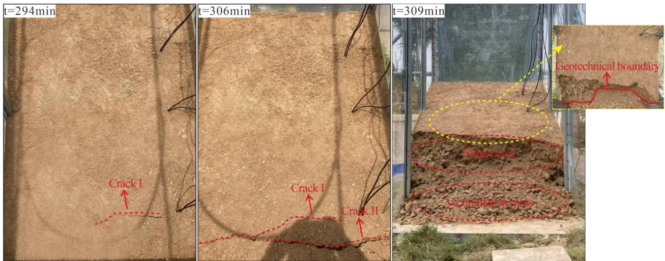
Figure 6. Deformation and failure process of the E2 slope.
