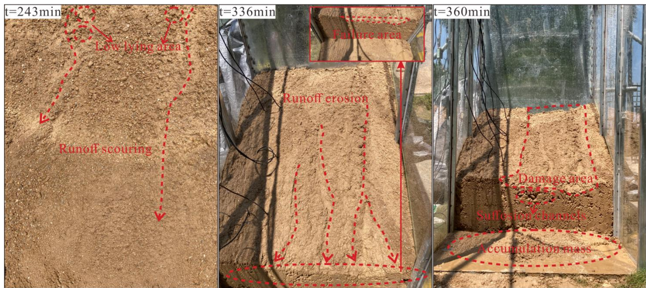
Figure 5. Deformation and failure process of the E1 slope.
