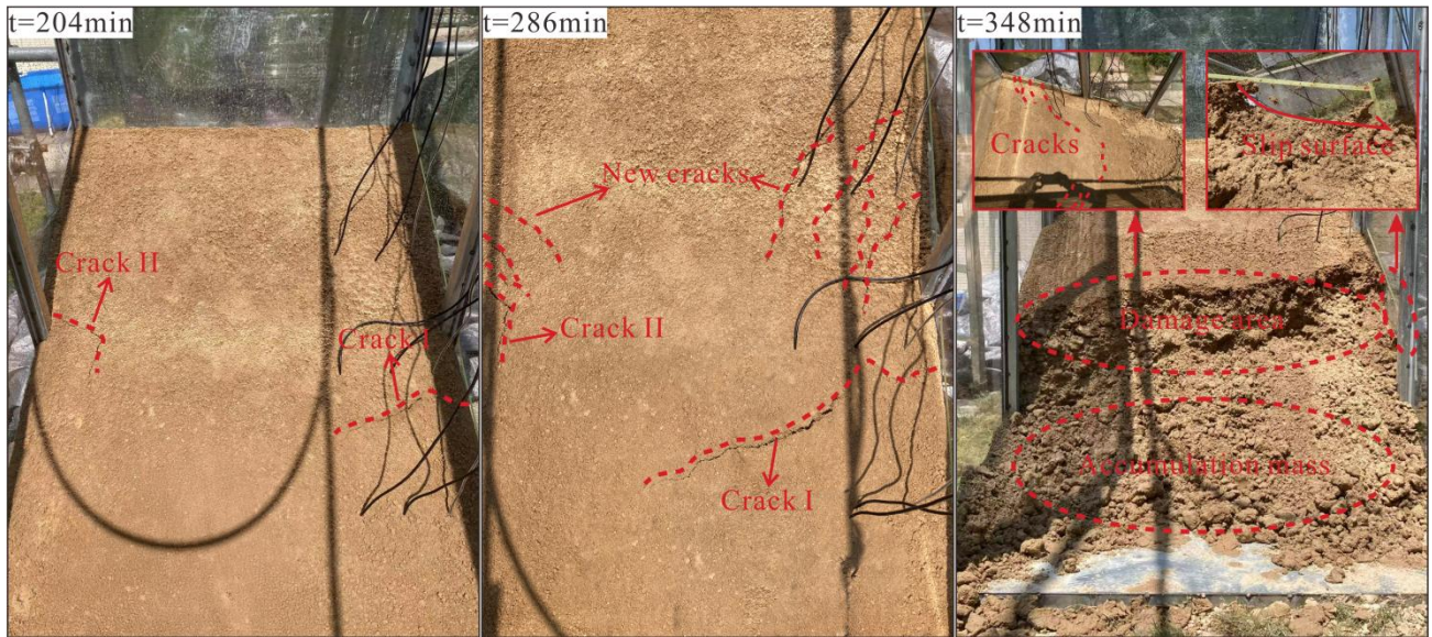
Figure 7. Deformation and failure process of the E3 slope.
