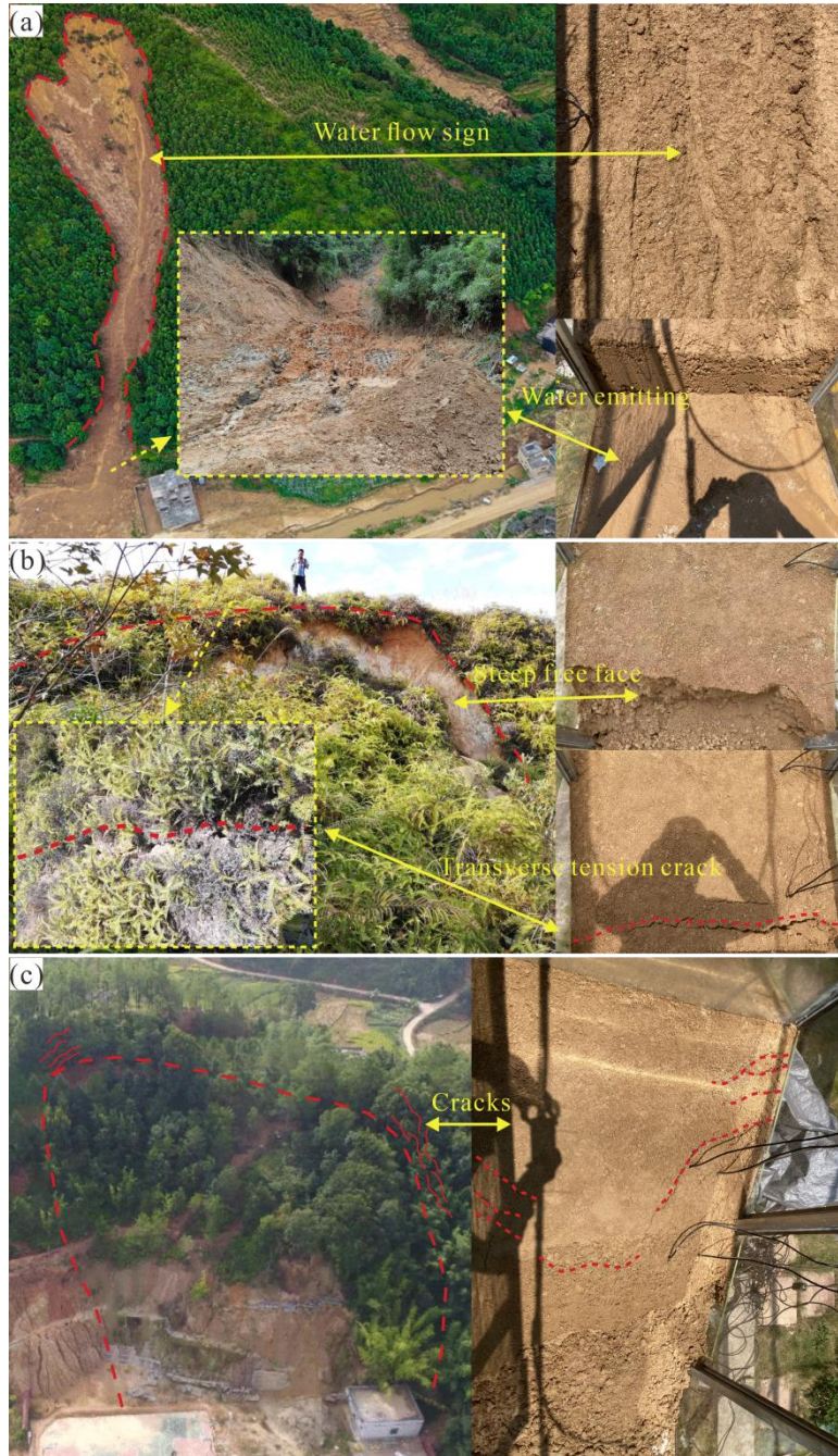
Figure 15. Comparison of Mibei landslides deformation with model tests. (a) E1 slope. (b) E2 slope. (c) E3 slope.
