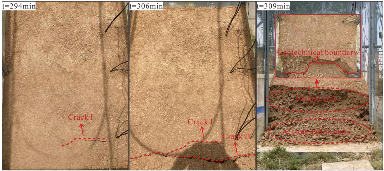
Figure 6. Deformation and failure process of the E2 slope.
