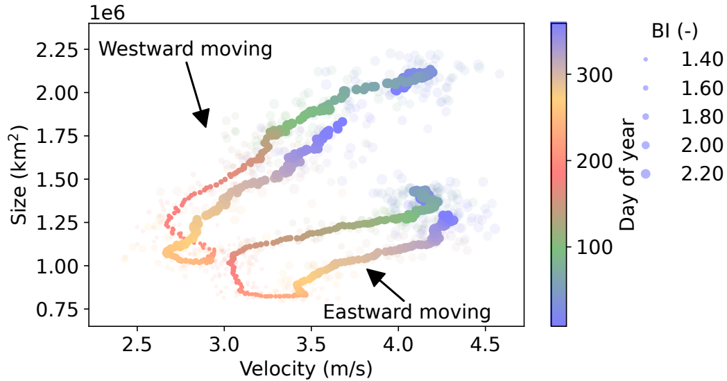
Figure 9. Climatological values per day of the year for size ( \text{km}^2 ) against absolute values of the propagation velocity ( \text{m/s} ). The scatter size indicates the blocking intensity (-), and the colour the day of the year. Each day of the year is averaged over the period of 1850-2014 over all 16 ensembles (light colours), and a 15-day running mean is plotted (opaque colours).
