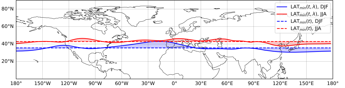
Figure 1. Difference between the longitude-dependent minimum latitude \text{LAT}_{\min}(t, \lambda) (continuous line), and the spatial-averaged minimum latitude \text{LAT}_{\min}(t) (dashed line). Both shown for winter (DJF, blue), and summer (JJA, red).
