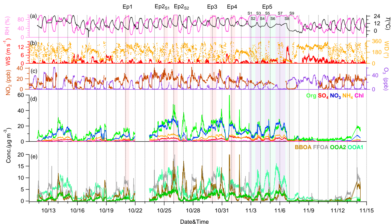
130 Figure 1. Time series of meteorological variables, gaseous species, and PM 1 species. In addition, five episodes (Ep1-5) with relatively high RH levels (> 95%) are marked for further discussion, with Ep5 being a 3-day consecutive fog event that was further divided into nine stages (S1-S9).
