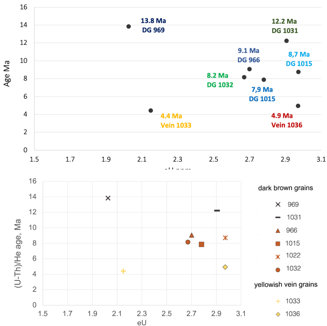
315 Figure 67. Goethite (U-Th)/He ages versus eU concentration of the samples. The effective modern uranium concentration (eU) was calculated based on the formulas given by (Flowers et al., 2023). DG means fragments of the dark grain; vein goethite from the yellowish vein material. Index is a sample ID in the Table 2.
