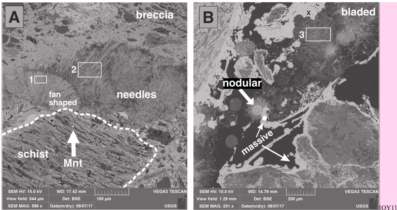
Figure 32. Backscatter SEM photomicrograph images of sample DR7-001 and DR7-002 from polished thin sections; (A) fan-shaped (26% Fe, 17% Mn for box 1), needle (28% Fe, 15% Mn for box 2), and massive cements of Fe and Mn oxides in the breccia part of sample DR-001; note schist grain in the lower left quadrant with a bright monazite grain (Mnt); (B) cement of breccia: bladed (box 3: 29% Fe, 35% Mn), nodular (white arrow: 33%
