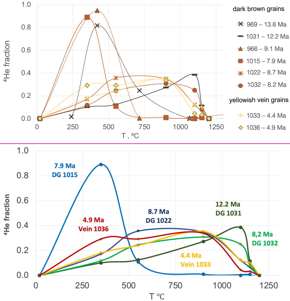
Fig. 56. Helium release pattern from the mainly (>95%) goethite grains sealed in Quartz ampoule. All measurements (with the exception of the samples 966 and 969; dotted line) were carried out under the same time-temperature conditions. DG means fragments of the dark grain; vein — goethite from the yellowish vein material. Index Values arcs a sample ID in the Table 2.
