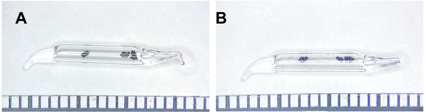
Figure 34. Fragments of goethite in a sealed quartz ampoule (A) before heating; (B) after heating. Scale bar 1 mm.
