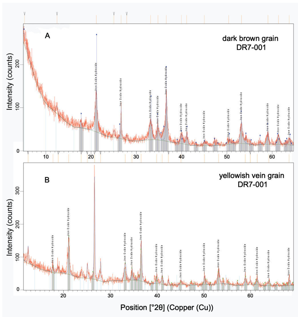
Figure 2. X-ray diffraction mineralogy of the dark brown clast (A), and yellow-brown vein material (B) from the DR7-001 sample. Iron Oxide Hydroxide peaks (marked grey) refers to the mineral goethite. The peaks of birnessite ( MnO_2 ) and quartz are observed in both samples. The yellow-brown vein material also contains minor amounts of plagioclase, and, probably, illite.
