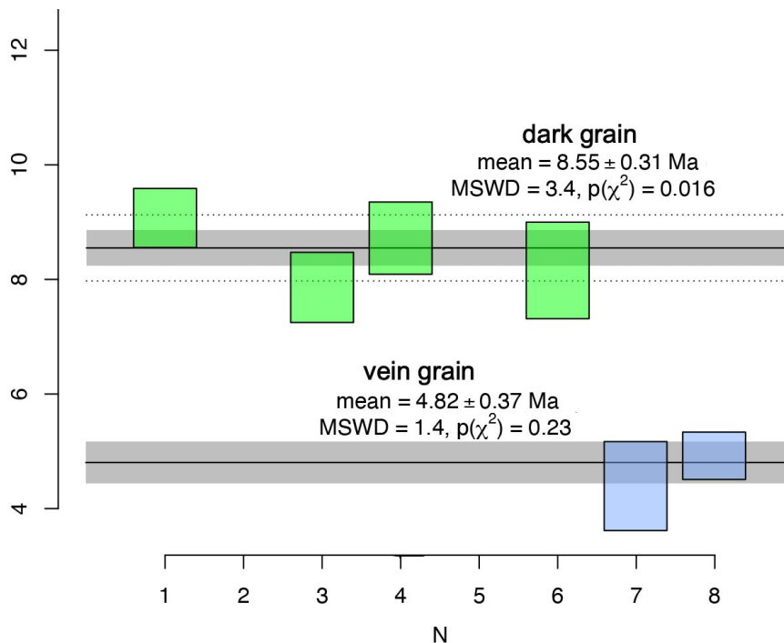
Figure 45. Results of (U-Th)/He dating of goethite from DR7-001 subsamples. Error bars 2 \sigma . Weighted mean plot constructed using IsoplotR software (Vermeesch, 2018).
