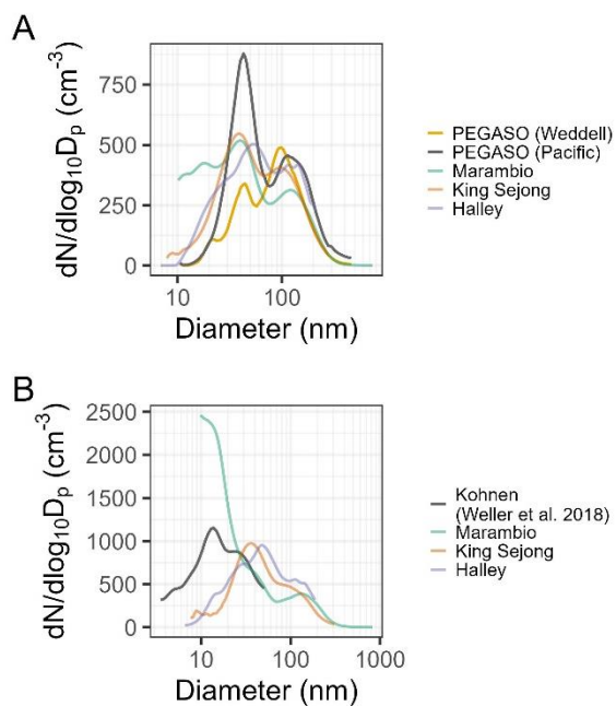
1185 Figure 6: PNSD intercomparisons: (a) PNSD from the PEGASO cruise both when influenced from air masses from the Weddell Sea and Pacific Ocean and the stations used for this study where overlapping data are available (Marambio, Halley and King Sejong stations), and (b) PNSD from the Kohnen station (Weller et al., 2018) and the stations used for this study where overlapping data are available (Marambio, Halley and King Sejong stations)
