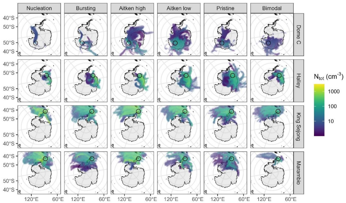
1180 Figure 5: Concentration weighted trajectory maps showing the sources of particles corresponding to each cluster at each site. 72 hour back trajectories calculated with HYSPLIT.
