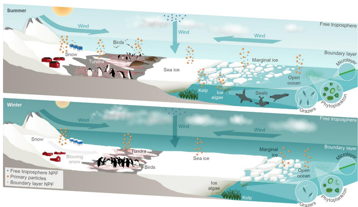
1195 Figure 7 Schematic illustrations of the sea ice, microbiota, sea-to-air emissions, and primary and secondary aerosols in Antarctica during summer (top) and winter (bottom).
