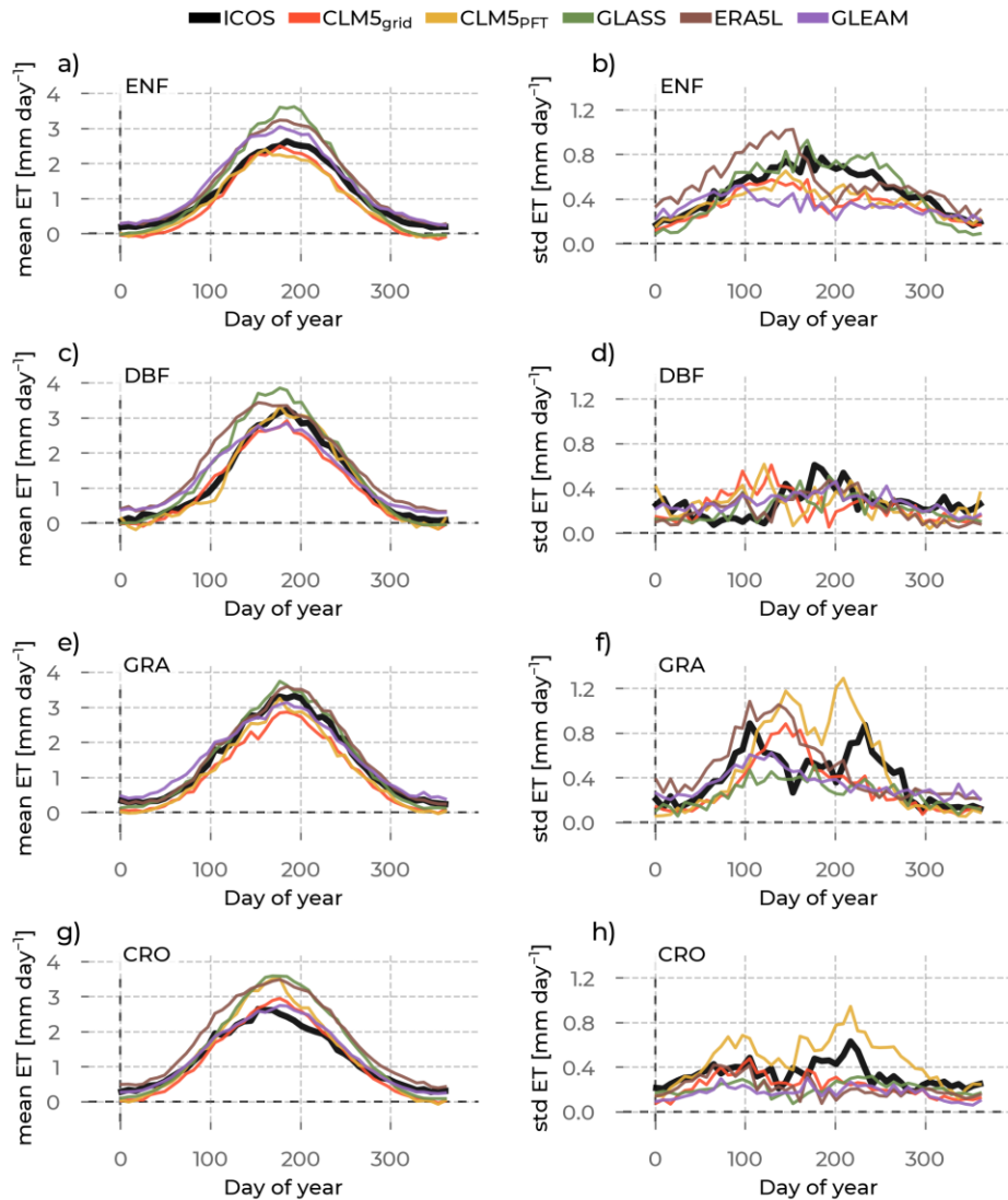
Figure 4: In the left column are the yearly evapotranspiration (ET) evolutions averaged across stations belonging to one plant functional type (rows: Evergreen Needleleaf Forest (ENF), Deciduous Broadleaf Forest (DBF), Grasslands (GRA), and Croplands (CRO)) and across the years (available years vary per station, see Supplementary Table S1). We differentiate the data source by color (Integrated Carbon Observation System (ICOS) observations: black, Community Land Model v5 (CLM5), CLM5 grid : red, CLM5 PFT : yellow, Global Land Surface Satellite (GLASS): green, European Center for Medium-Range Weather Forecasting Reanalysis 5 – Land
