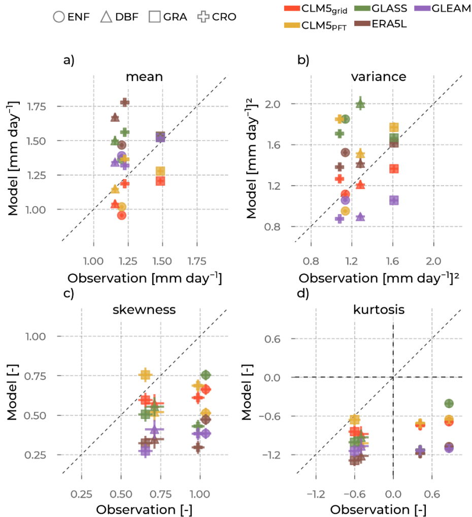
Figure 9: The mean (a), variance (b), skewness (c), and excess kurtosis (d) of the evapotranspiration (ET) distributions (visualized in Figure 8) from the models (y-axis, colors: Community Land Model v5 (CLM5), CLM5 grid: red, CLM5PFT: yellow, Global Land Surface Satellite (GLASS): green, European Center for Medium-Range Weather Forecasts Reanalysis 5 Land (ERA5L): brown, Global Land Evaporation Amsterdam Model (GLEAM): purple), as opposed to the corresponding values from observations (x-axis) aggregated for each plant functional type (marker type): Evergreen Needleleaf Forest (ENF), Deciduous Broadleaf Forest (DBF), Grasslands (GRA), Croplands (CRO). The error bars are the standard errors of the respective moment, depending on the sample size.
