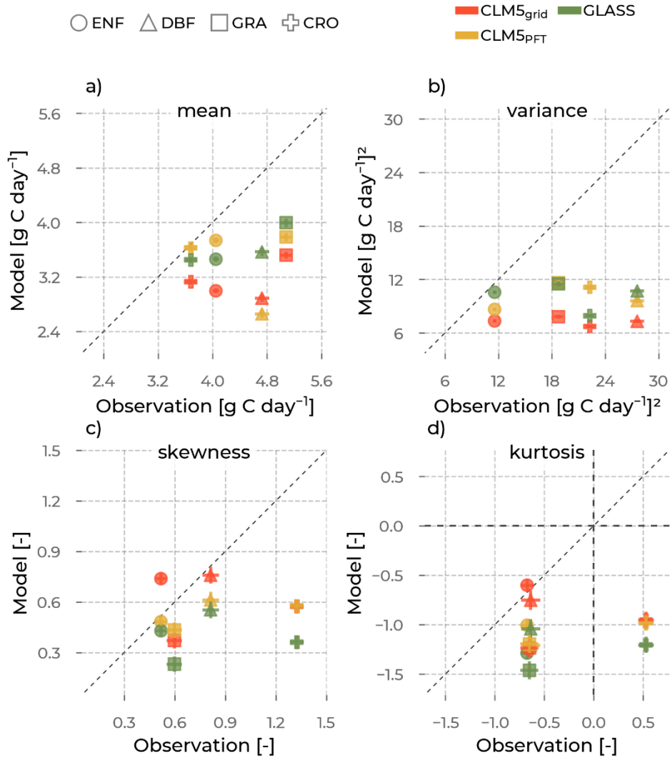
Figure 11: The mean (a), variance (b), skewness (c), and excess kurtosis (d) of the gross primary production (GPP) distributions (visualized in Figure 10) from the models (y-axis, colors: Community Land Model v5 (CLM5), CLM5 grid: red, CLM5PFT: yellow, Global Land Surface Satellite (GLASS): green), as opposed to the corresponding values from observations (x-axis) aggregated for each plant functional type (marker type): Evergreen Needleleaf Forest (ENF), Deciduous Broadleaf Forest (DBF), Grasslands (GRA), Croplands (CRO). The error bars are the standard errors of the respective moment, depending on the sample size.
