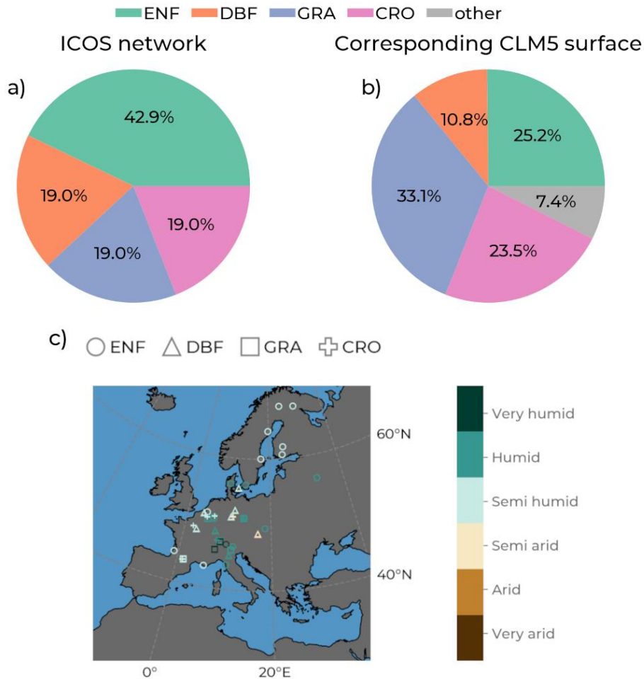
Figure 1: The share of represented plant functional types (by color: Evergreen Needleleaf Forest (ENF, green), Deciduous Broadleaf Forest (DBF, orange), Grasslands (GRA, purple), and Croplands (CRO, pink)) in a) in the ICOS station network used in subsequent analyses and b) in the corresponding grid cells in our European CLM5 setup. In c) is a map showing the locations of the ICOS stations, with the marker type indicating their PFT and the color of the marker indicating their hydro-climate (adapted from Jafari et al. (2018)) based on the mean annual precipitation from the Consortium for Small-Scale Modeling (COSMO) -Reanalysis 6. Our 3 km European CLM5 simulation domain corresponds to the entire map box in c).
