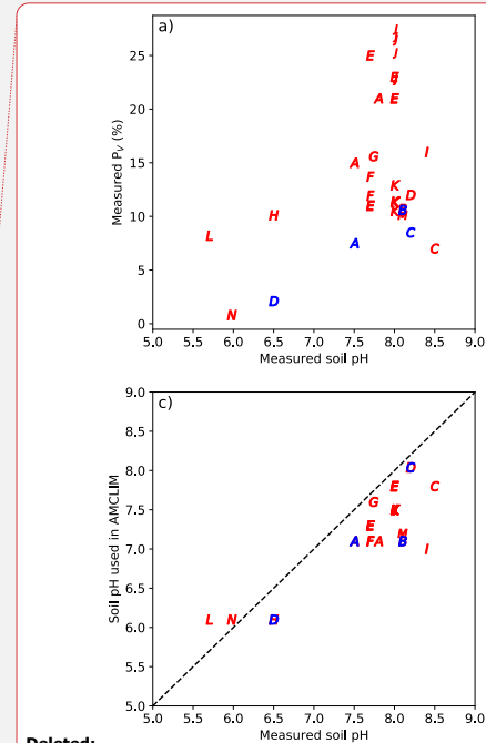
815 Figure 14. Measured percentage volatilization rates ( P_v , %) vs. measured soil pH (a). Modelled P_v vs. soil pH used in AMCLIM (b). Soil pH used in AMCLIM compared with measured soil pH (c), with black dashed line the 1:1 line.
