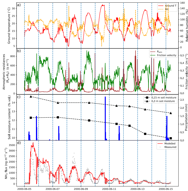
495 Figure 5. Meteorological variables measured by GRAMINAE and site simulations for \text{NH}_3 emissions from a post-cutting grassland after fertilization in Braunschweig, Germany, from 5 June 2000 to 15 June 2000 by AMCLIM-Land. (a) Surface temperature and
