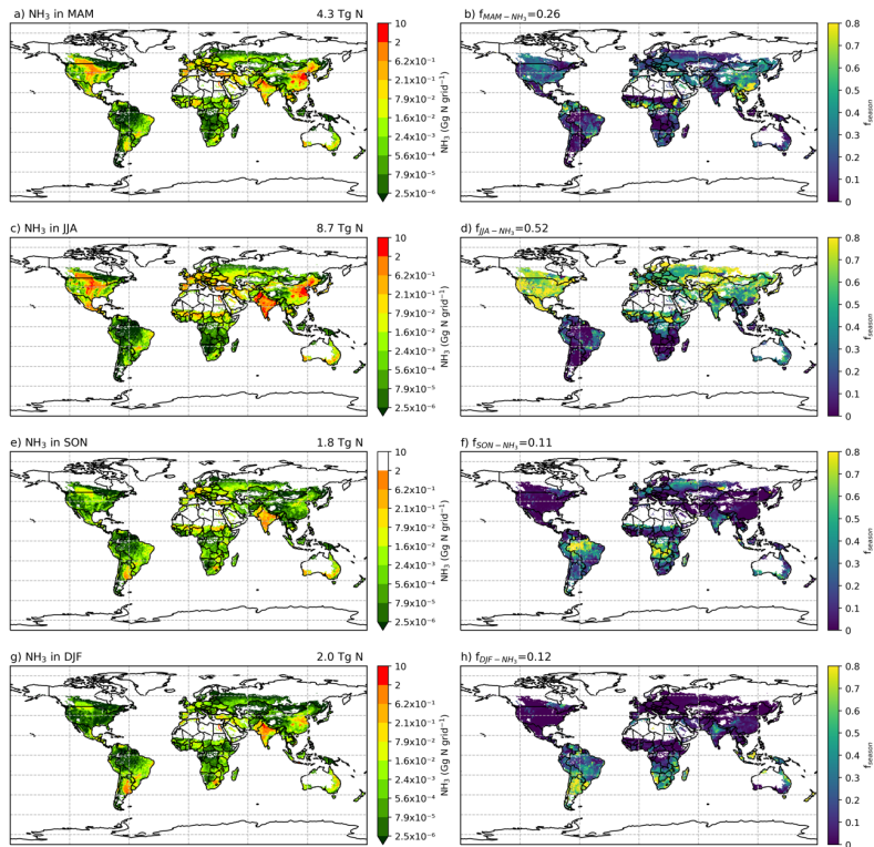
Figure A4. Same as Fig. 10 but for 2018.
