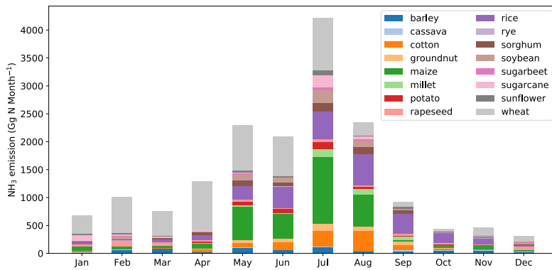
Figure A5. Same as Fig. 11 but for 2018.
