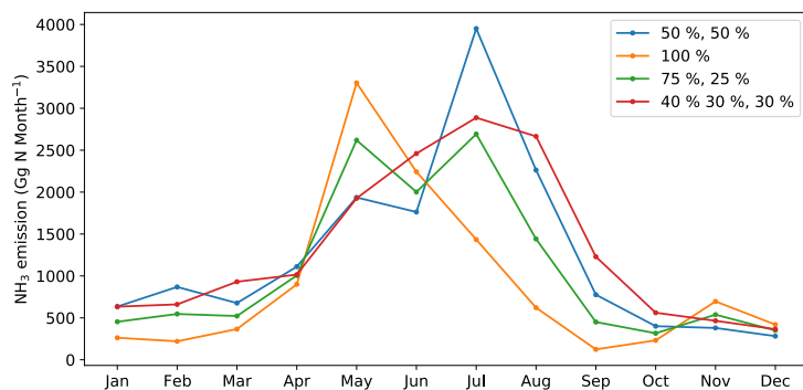
205 Figure A15. Simulated global monthly \text{NH}_3 emissions ( \text{Gg N month}^{-1} ) from synthetic fertilizer use in 2010 using the four different fertilization scenarios.
