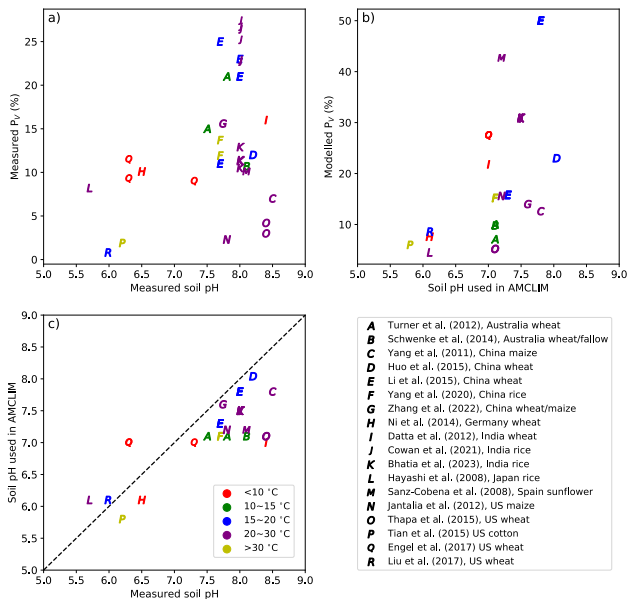
815 Figure 14. Measured percentage volatilization rates ( P_v , %) vs. measured soil pH (a). Modelled P_v vs. soil pH used in AMCLIM (b). Soil pH used in AMCLIM compared with measured soil pH (c), with black dashed line the 1:1 line.
