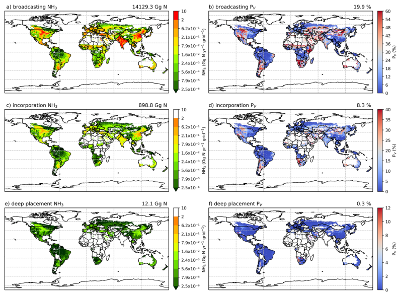
Figure A9. Simulated \text{NH}_3 emissions (Gg N yr -1 ) from synthetic fertilizer application by three techniques and the corresponding volatilization rates ( P_v ) in 2010. \text{NH}_3 emissions from (a) broadcasting, (c) incorporation and (e) deep placement. Percentage of applied N that volatilizes as \text{NH}_3 by (b) broadcasting, (d) incorporation and (f) deep placement.
