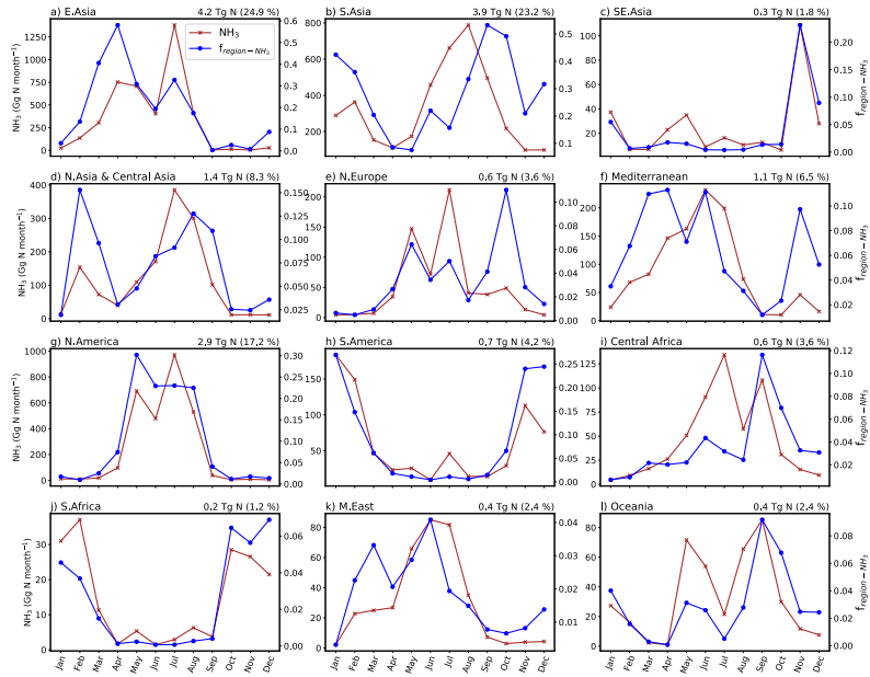
160 Figure A6. Same as Fig. 12 but for 2018.
