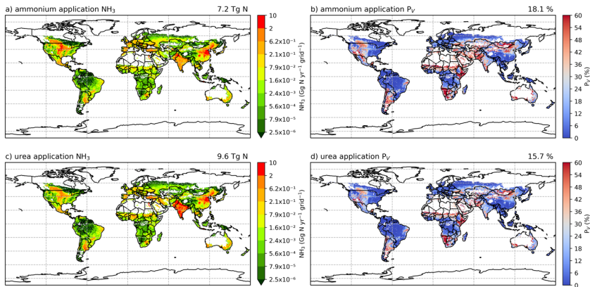
Figure A3. Same as Fig. 8 but for 2018.
