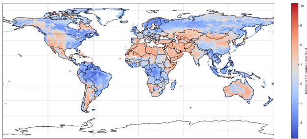
Figure A12. Global soil pH. Data from HWSO v1.2 (Wieder et al., 2014).
