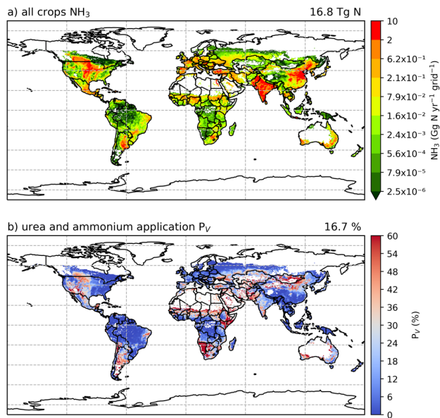
Figure A2. Same as Fig. 7 but for 2018.
