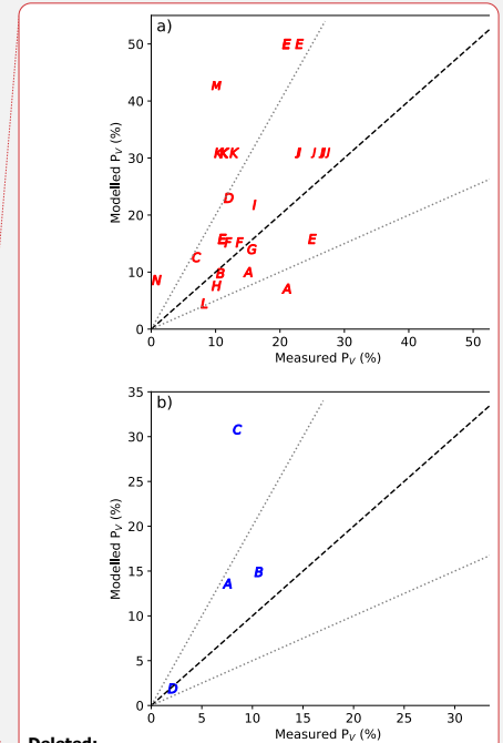
Figure 13. Modelled percentage volatilization rates ( P_v , %) compared with experimental studies (Hayashi et al., 2008; Sanz-Cobena et al., 2008; Yang et al., 2011; Datta et al., 2012; Jantalia et al., 2012; Turner et al., 2012; Ni et al., 2014; Schwenke et al., 2014; Huo et al., 2015; Li et al., 2015; Tian et al., 2015; Thapa et al., 2015; Engel et al., 2017; Liu et al., 2017; Cowan et al., 2021; Zhang et al., 2022; Bhatia et al., 2023). Measurement data were from literature that studied \text{NH}_3 volatilization from (a) urea application and (b) ammonium fertilizer application to field. Black dashed line is the 1:1 line, and grey dotted lines indicate the values within a factor of 2. AS: ammonium sulfate; CAN: calcium ammonium nitrate.
