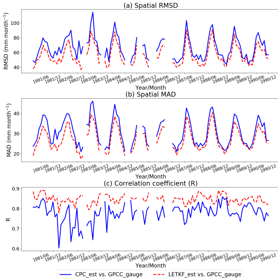
Figure 5: The time series of (a) the spatial root mean square difference (RMSD; \text{mm month}^{-1} ), (b) the spatial mean absolute difference (MAD; \text{mm month}^{-1} ) and (c) Pearson's correlation coefficient (R), verified against the GPCC_gauge. The blue solid and red dashed lines represent the CPC_est and LETKF_est, respectively. The validations are not performed for the months in which we skipped the estimation for daily precipitation (Jan., 1981; Apr., 1983; Jan., 1984; Jan. –Feb. and Jul. –Aug., 1985; Jan., Mar., Sep. and Nov., 1986).
