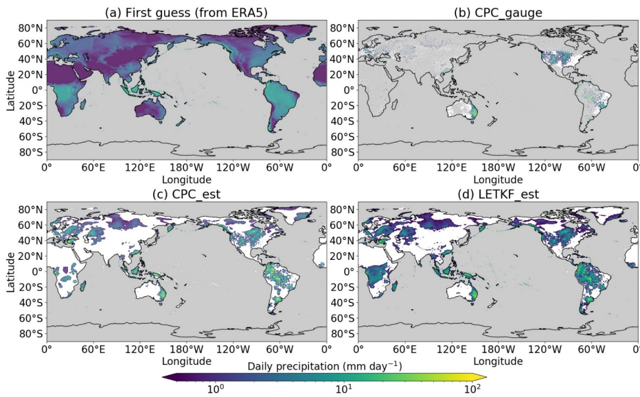
Figure 3: An example of the precipitation fields ( \text{mm day}^{-1} ) for (a) the first guess used in our study, (b) the rain gauge observations of CPC_gauge, and the global precipitation estimates of (c) CPC_est and (d) LETKF_est (on Nov. 15th, 1988). Pixels on the ocean are colored in gray for all subplots, as well as those where no rain gauge observations are available for subplot (b). Pixels are colored in white when the precipitation is < 0.5 \text{ mm day}^{-1} .
