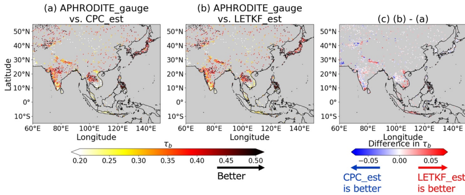
325 Figure 8: Kendall's rank correlation coefficient ( \tau_b ) computed against the daily precipitation of APHRODITE_gauge for (a) CPC_est and (b) LETKF_est at each pixel. Subplot (c) represents the difference between (b) and (a). Darker colors in (a–b) indicate that the precipitation estimates are more similar to APHRODITE_gauge. Warm colors in (c) indicate that LETKF_est is more similar to APHRODITE_gauge than CPC_est, and cold colors indicate otherwise. \tau_b is computed only at pixels where more than 1,800 samples from APHRODITE_gauge are available, and the pixels are 330 colored in gray if they do not match this condition.
