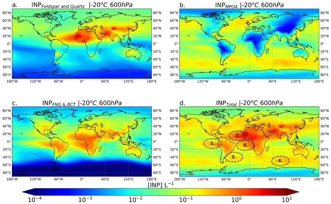
1285 Figure 5: Multi-year mean distributions calculated by TM4-ECPL for INP number concentrations derived from dust (a), MPOA (b), PBAP (c), and the sum of the aforementioned INP (d) at a pressure level of 600 hPa for an activation temperature of -20^{\circ}\text{C} . Circles labelled 1 to 5 indicate areas of interest, with numbering details provided in the main text.
