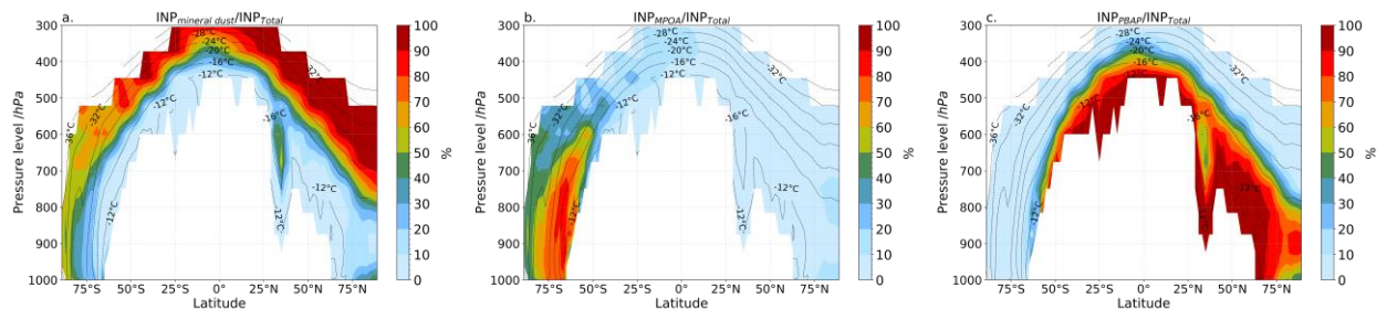
Figure 7: Multi-annual averaged zonal mean profiles of the percentage contribution of each species to the total INP number concentration, calculated at modelled ambient temperature by TM4-ECPL and plotted only where INP number concentration is larger than 10^{-5} \text{ L}^{-1} (i.e. 0.01 \text{ m}^{-3} ), showing contributions from (a) mineral dust, (b) marine bioaerosols and (c) fungal spores and bacteria (PBAP). Black dashed contour lines represent the model's annual mean temperature.
