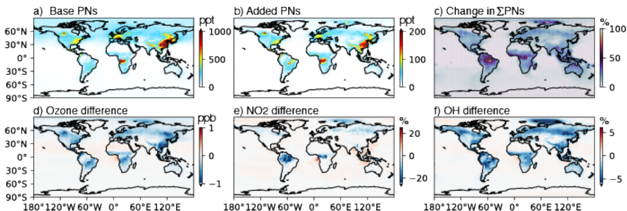
Figure 8 – Global average surface concentrations at 2 \times 2.5^\circ from May 1 to June 10, 2016 for a) base PNs = PAN, MPAN, PPN, and BZPAN (Table 4), b) added PNs = PHAN, LIMPAN, PINPAN, AROMPN, MEKPN, APAN (Table 4), c) percentage change in the revised model (Base + added PNs) compared to the base model, d) difference in surface ozone, e) difference in surface \text{NO}_2 , and f) difference in surface OH.
