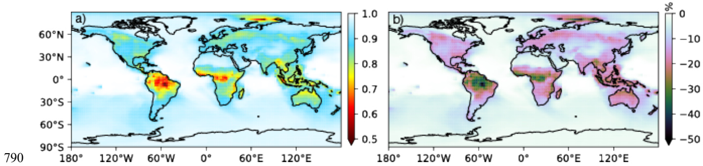
Figure 9 – a) Modeled global average fraction of commonly measured PNs (PAN, MPAN, PPN) compared to \sum PNs (PAN, MPAN, PPN, BZPAN, PHAN, LIMPAN, PINPAN, AROMPN, MEKPN, APAN). b) Reduction in commonly measured PNs vs. \sum PNs in the revised model simulation (Section 5) compared to the base simulation (approximately 100%).
