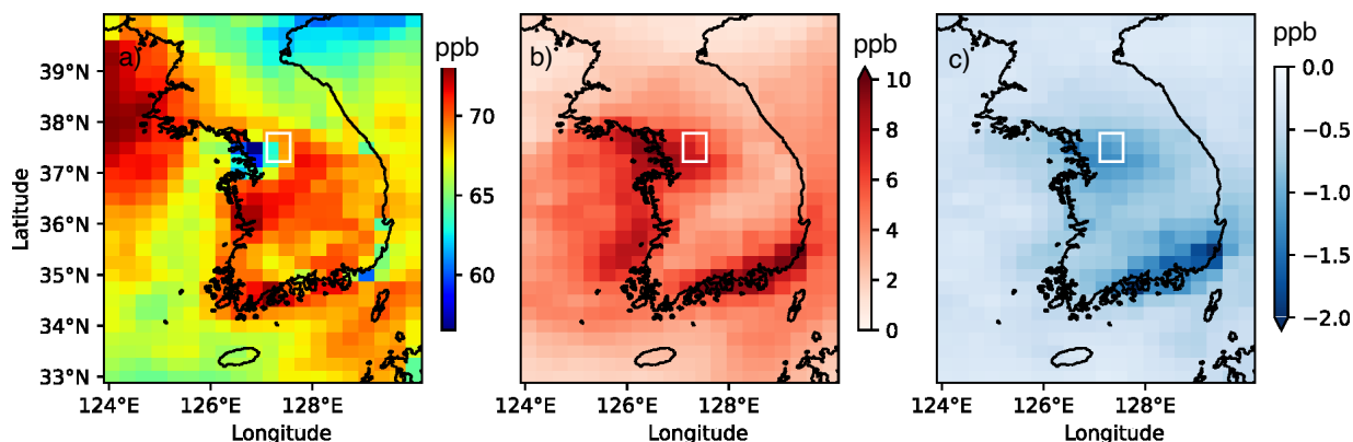
Figure 5 – a) Maximum daily eight-hour average (MDA8) ozone from May 1 to June 10, 2016, and the impact from b) scaled VOCs as described in Section 2 and c) adding peroxyxynitrate (PN) chemistry to the simulation in b) described in Section 5. The white box designates the Seoul Metropolitan Area (SMA).
