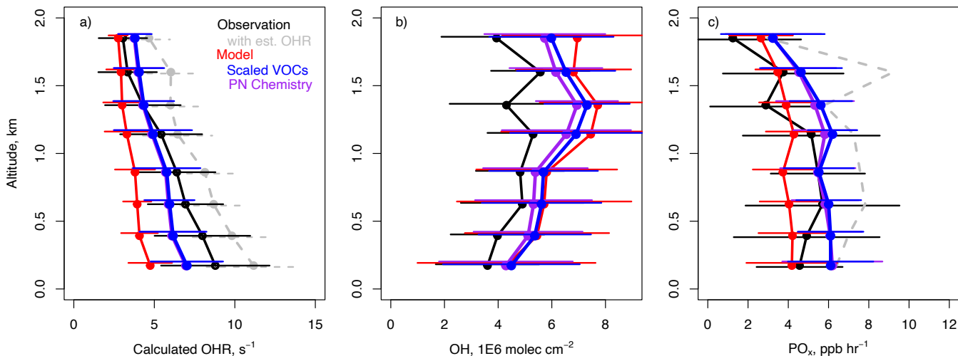
Figure 1 – Mean vertical profile and standard deviation in the Seoul Metropolitan Area (SMA) (127.1 to 127.7°E, 37.2 to 37.7 745 °N) from May 1 to June 10, 2016, for data collected after 11 am local time for a) calculated OH reactivity (OHR) for VOCs + CO (Table 1), b) OH, and c) net production of O_x ( PO_x=O_3 + NO_2 ). Data are averaged into 8 bins of approximately 240 m for the observations (black), the base model (red), the model with scaled VOCs (blue), and improved peroxyxynitrate (PN) chemistry (purple). Calculation of OHR, the inclusion of estimated missing OHR (est. OHR), and net PO_x , and descriptions of model simulations are given in Sections 3 and 4.
