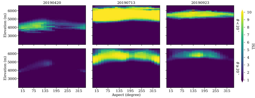
Figure 4. TSI values at different elevation (y-axis), aspect (x-axis) and slope classes (top row: flat slope with \theta < 20^\circ , bottom row: step slope with \theta > 20^\circ ) for Hunza basin. Three observation dates in spring (left column), summer (middle column) and late autumn (right column) are displayed. Aspect of 0, 90, 180 and 270 degrees align with the north, east, south and west direction, respectively.
