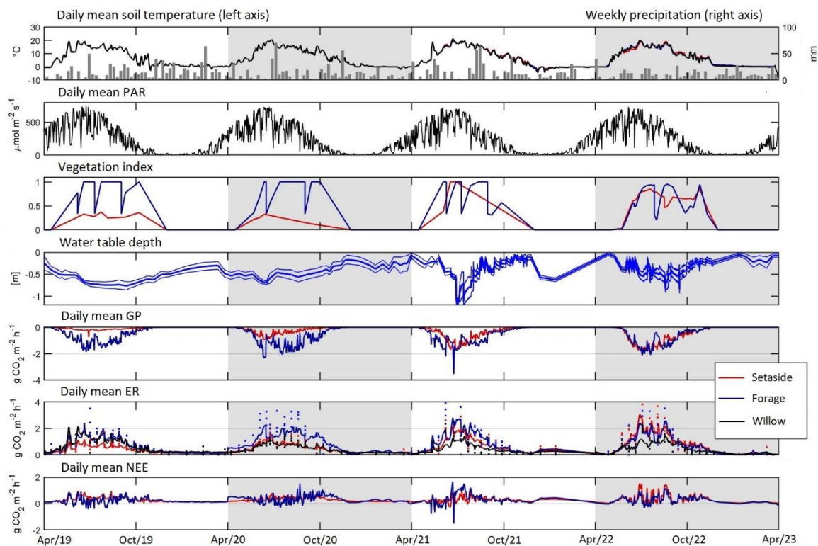
311 Figure 1: Daily mean of soil temperature and precipitation, photosynthetically active radiation (PAR), 312 vegetation index, 313 water table depth (site mean±std), gross photosynthesis, measured (dots) and model predicted (line) ecosystem respiration 314 (soil respiration for willow) and net ecosystem exchange. Annual modelling periods (Apr - Mar) are marked with light grey or white background.
