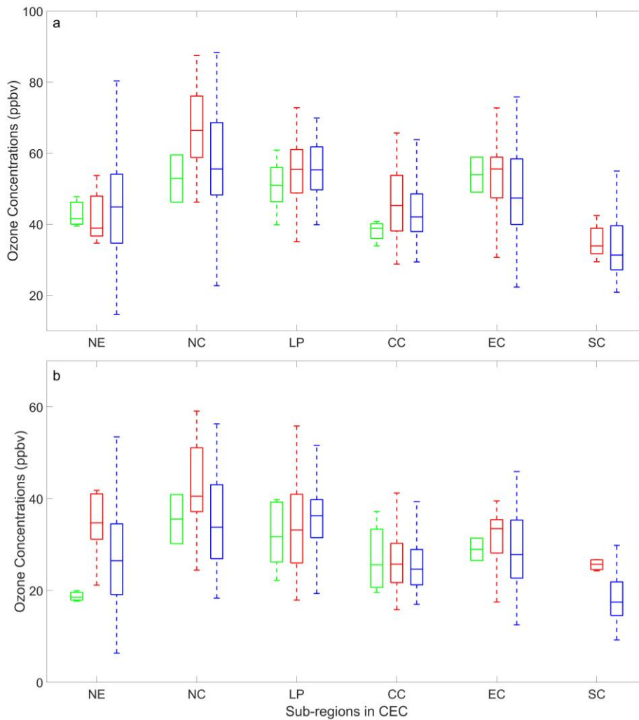
410 Figure 7: Boxplots of near-surface ozone concentrations during daytime (a) and nighttime (b) in six sub- regions for the periods of DSI (green) and IST (red) and intrusion-free conditions (blue). Boxes indicate the distribution of near-surface ozone concentrations between the 25th and 75th percentiles, with the horizontal lines inside the boxes denoting the median O3 concentrations. 9 direct SI samples affecting LP, and 2-4 samples affecting the remaining five sub-regions over CEC, are used to perform the statistical analysis.
