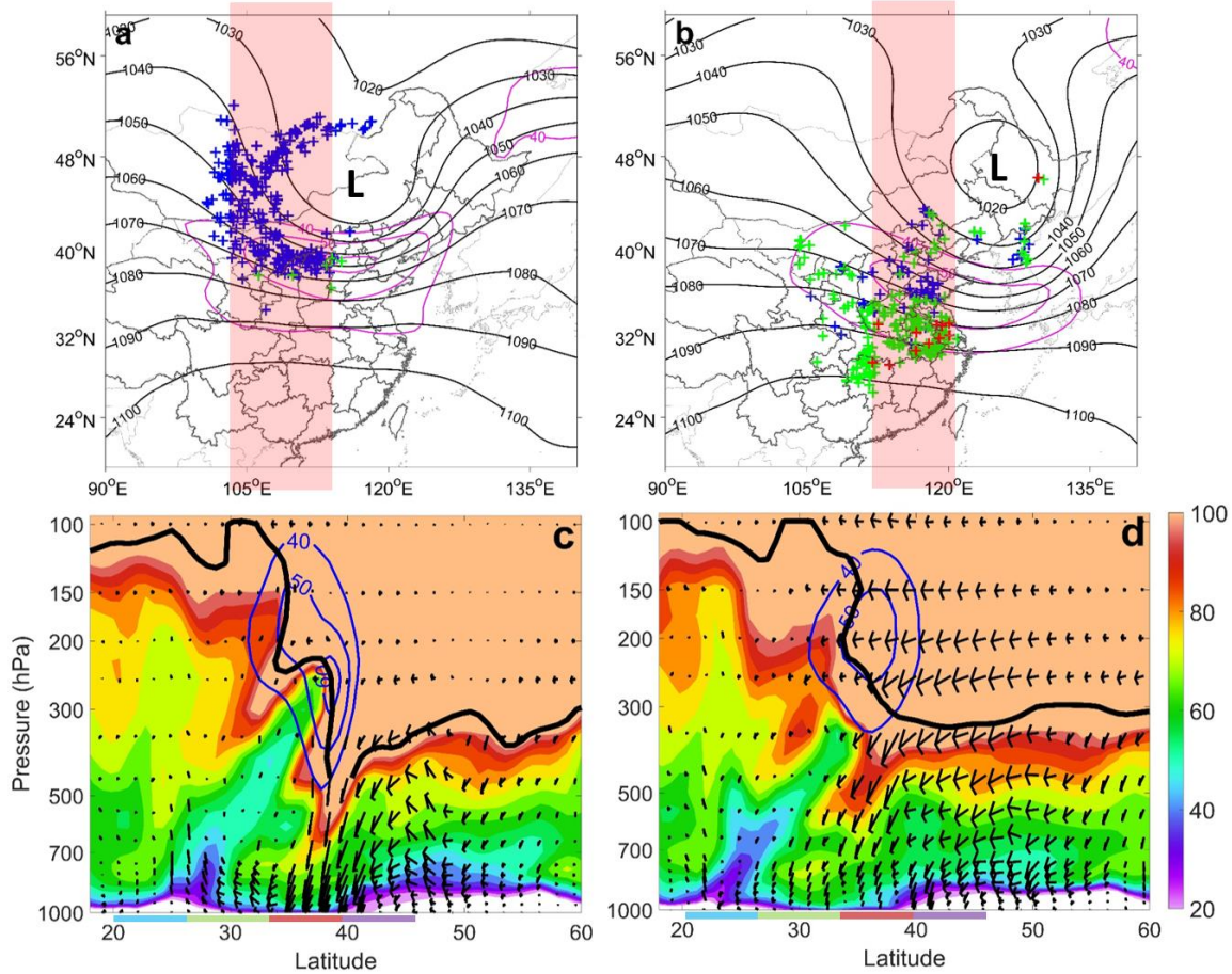
540 Figure 11: 300-hPa geopotential height (gpdm, black lines) and U-component of horizontal wind at 200 hPa (> 40 m s -1 , magenta lines) at (a) 20:00 on May 19 and (b) 20:00 on May 20, 2019. The plus signs in Figures a and b represent the position of stratospheric air particles in the middle troposphere (blue), the lower troposphere (green) and below 500 m (red), respectively. Vertical cross section of wind speed (> 40 m s -1 , blue lines) and O 3 concentrations (ppb, color contours) averaged along the red square in Figures a and b on (c) May 19 and (d) May 20, 2019. The thick solid black line in Figures c and d indicates the PV of 1.5 PVU. The arrows in Figures c and d are the V-W (meridional) wind fields. The bottom lines of purple, red, green and blue in 545 Figures c and d indicates the sub- regions NE, NC and LP, CC and EC, and SC, respectively.
