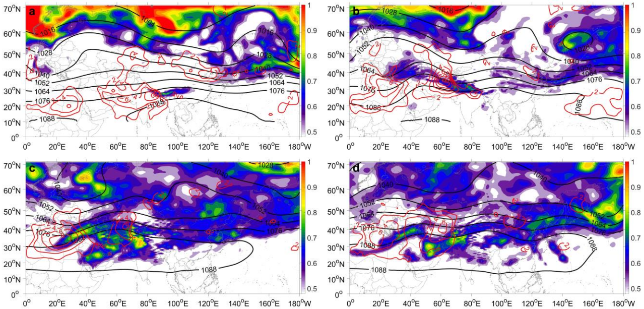
Figure 10: 400 hPa PV (PVU, color contours), geopotential height (gpm, black lines), and vertical velocity (>0 hPa s -1 , red lines) averaged at heights of 150–400 hPa in May (a), June (b), July (c) and August (d) in 2019.
