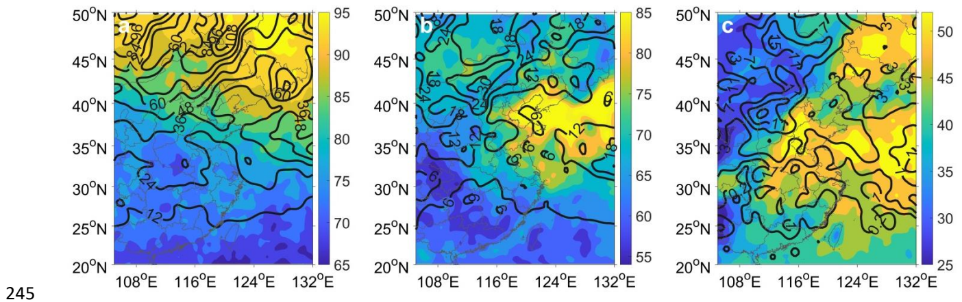
Figure 2: Spatial correspondence between SI ozone (ppbv, black contours) and actual tropospheric ozone from the OMI remote sensing data (ppbv, color contours) from May to August 2019 at altitudes of a) 400, b) 600, and c) 850 hPa.
