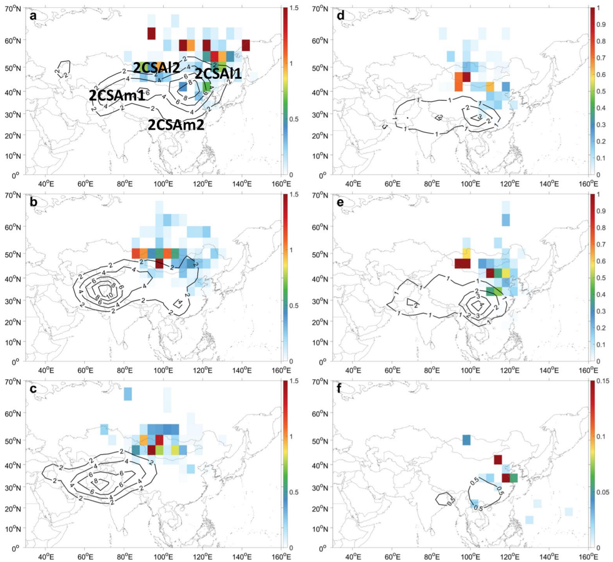
Figure 8: Same as Fig. 7 but for DSI.
