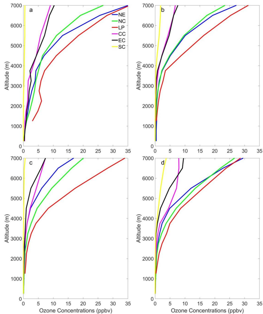
230 Figure 3: Vertical profiles of contributions of stratospheric ozone (ppbv) directly transported to the troposphere over six sub-regions of CEC from May to August in 2019: a) May, b) June, c) July, d) August. The altitude is above sea level (a.s.l.).
