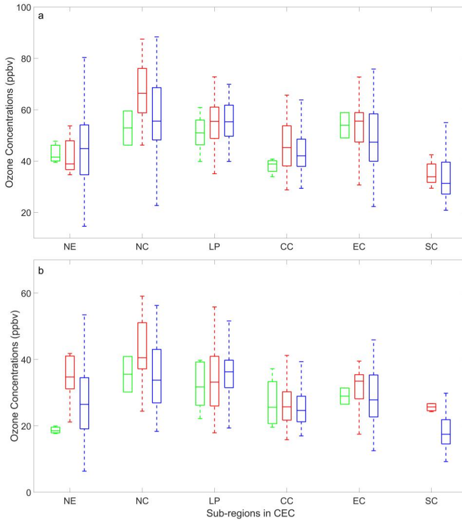
Figure 6: Boxplots of near-surface ozone concentrations during daytime (a) and nighttime (b) in six sub- regions for the periods of DSI (green) and IST (red) and intrusion-free conditions (blue). Boxes indicate the distribution of near-surface ozone concentrations between the 25th and 75th percentiles, with the horizontal lines inside the boxes denoting the median O3 concentrations. 9 direct SI samples affecting LP, and 2-4 samples affecting the remaining five sub-regions over CEC, are used to perform the statistical analysis.
