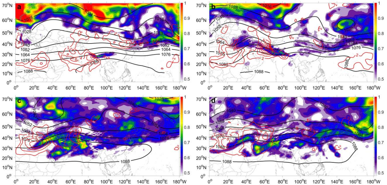
430 Figure 9: 400 hPa PV (PVU, color contours), geopotential height (gpm, black lines), and vertical velocity (>0 hPa s -1 , red lines) averaged at heights of 150–400 hPa in May (a), June (b), July (c) and August (d) in 2019.
