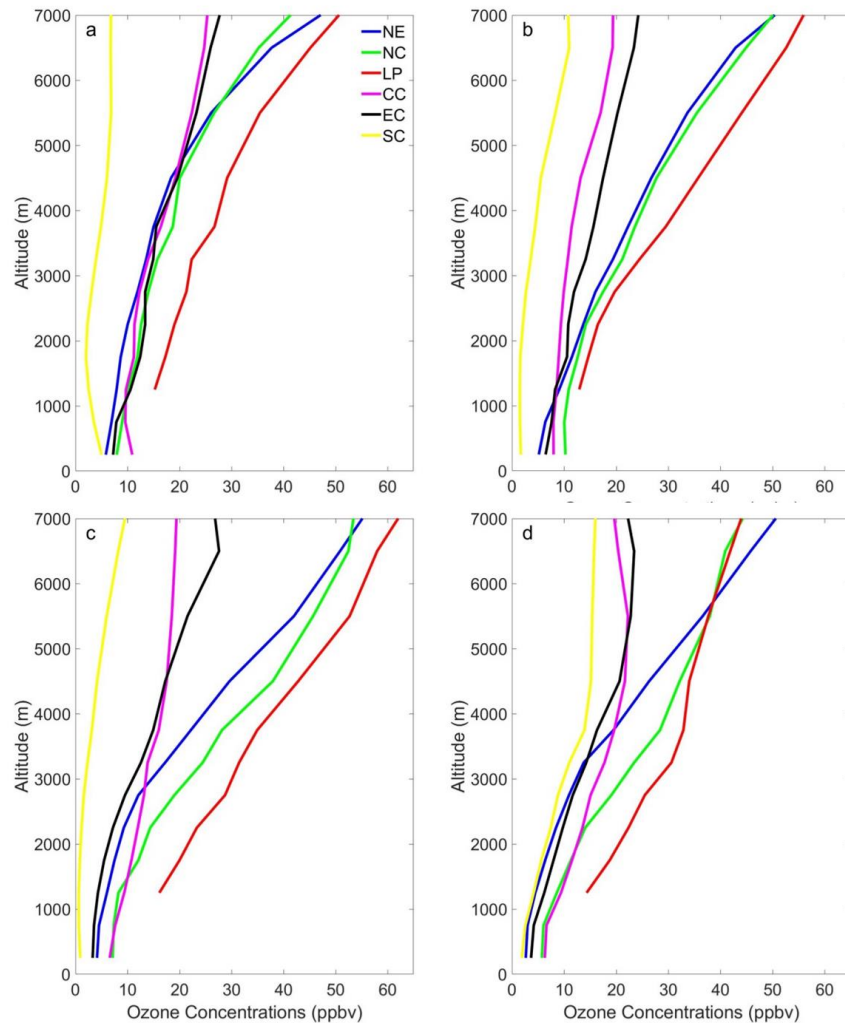
250 Figure 4: Same as Fig. 3 but for indirect transport.
