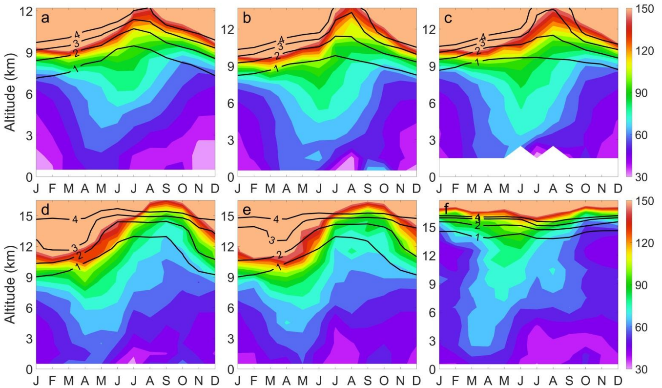
Figure 2: Monthly variations of vertical O 3 concentrations (ppbv) of TOST averaged during 1990-2019 for a) NE, b) NC, c) LP, d) CC, e) EC and f) SC. The black lines are PV isolines of 1-4 PVU.
