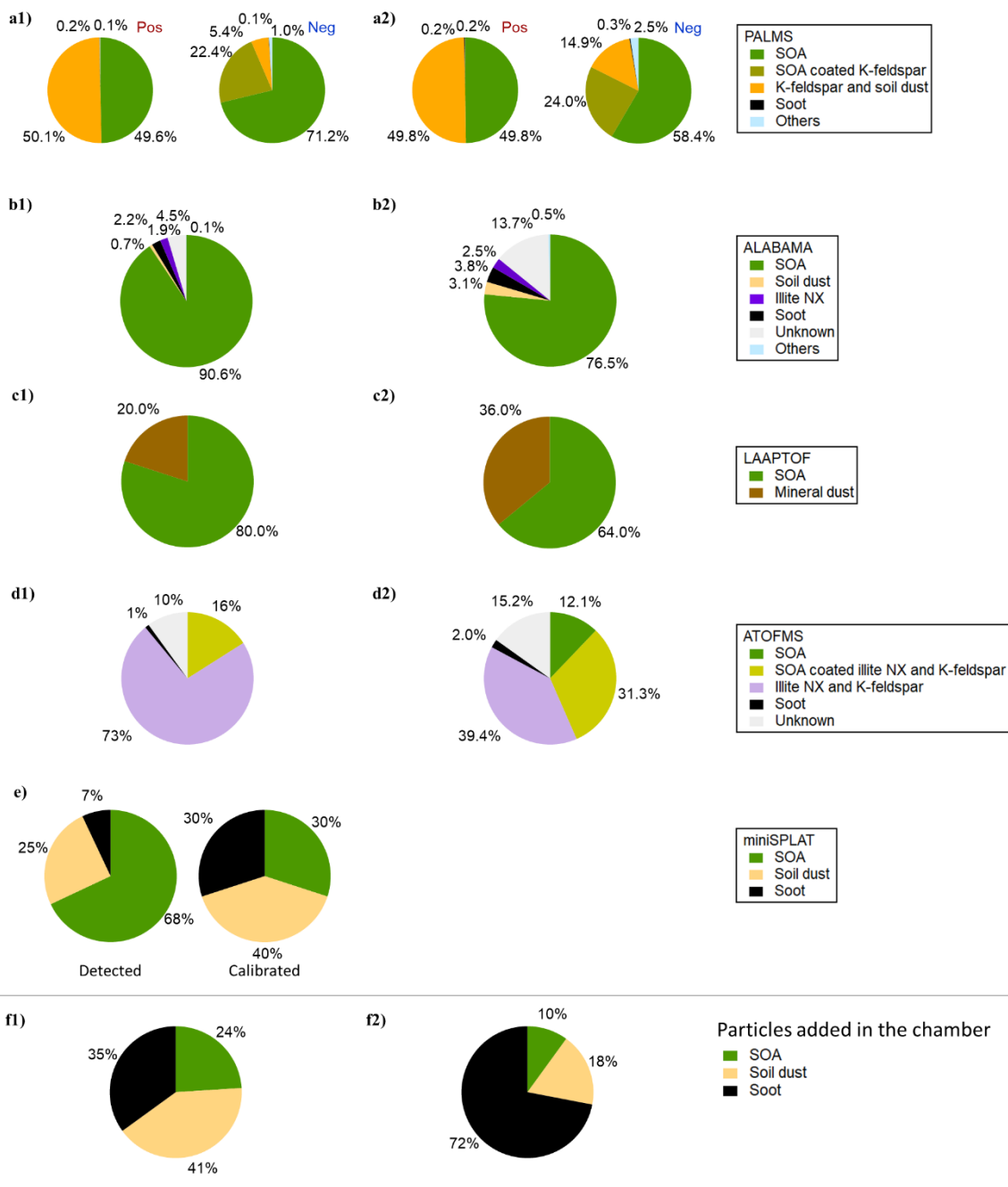
Figure 109: Particle classes and their relative contributions for blind periods P1 and P2 for: a1-2) PALMS, b1-2) ALABAMA, c1-2) LAAPTOF, d1-2) ATOFMS and e) miniSPLAT (which only reported data in P1). f1-2) are the same pie charts as those in Fig. 1, added here for better comparison. The plots shown here are the data provided to the referees after experiments (i.e., before participants knew the composition of the blind experiment). Note the left pie chart for miniSPLAT represents acquired mass spectra, consistent with what is presented for the other SPMSs. The right pie chart, provided to the referees after experiments, represents calibrated data (see text for details). Particle clustering is shown for positive and negative spectra separately for the unipolar switchable PALMS instrument.
