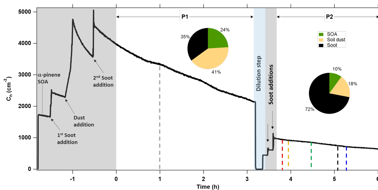
865 Figure 2: Time series of total particle C_n measured by a CPC in the APC chamber during the blind experiments. SPMS measurements were conducted during two periods, P1 and P2. In P1, the SPMSs started sampling at the same time (grey dashed line), except miniSPLAT which started 15 min later. In P2, sampling started at different times (red, orange, green, black and blue dashed lines are for PALMS, ATOFMS, LAAPTOF, miniSPLAT and ALABAMA, respectively). The pie charts denote particle types and their number fractions in P1 and P2, respectively. Note that the grey and blue shaded areas denote the aerosol mixture preparation periods, and a dilution step when the chamber was partly pumped out and refilled with clean air.
