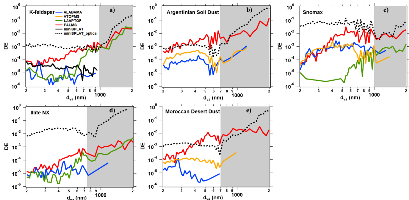
Figure 43: Detection efficiencies of SPMSs for selected particle types, i.e., a) K-feldspar, b) Argentinian soil dust, c) Snomax, d) Illite NX, and e) Moroccan desert dust, as a function of the d_{va} measured by ALABAMA (blue), ATOFMS (orange), LAAPTOF (green), PALMS (red), and miniSPLAT (black). Note that the uncertainty for super-micrometer particles is larger due to the low number concentration of these particles in the experiments. The DE curves in white and shaded area are based on SMPS and APS results, respectively. There were overlap results between SMPS and APS for the sizes around 700 nm to 1 \mu\text{m} d_{va} . In such an overlap range, we chose SMPS data as reference to calculate DE. Given different shape factors and particle densities, the conversions of d_m and d_{ca} to d_{va} were different for different particle types. Therefore, the end point of SMPS based result or shift point between white and shaded area varies from sample to sample. Note that the DE of miniSPLAT is defined differently from the other SPMSs. The sized distribution derived DE (dashed black) and the hits only derived DE (solid black) for K-feldspar is shown to provide the upper and lower limits of miniSPLAT DE (see text for details).
