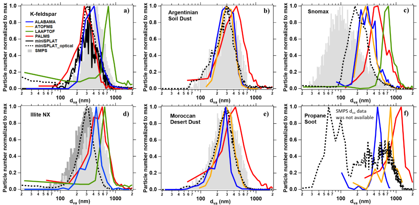
Figure 32: SPMS size distributions (normalized to maximum particle number) for selected particle types, i.e., a) K-feldspar, b) Argentinian soil dust, c) Snomax, d) Illite NX, e) Moroccan desert dust, and f) Propane soot. Color codes correspond to d_{va} measured by ALABAMA (blue), ATOFMS (orange), LAAPTOF (green), PALMS (red), and miniSPLAT (black). Note that the dashed black curves represent the DE of the size distribution measured by miniSPLAT, while in a) the solid black curve represents DE consistent with the other SPMSs (see text for details). Particle sizes measured by the SMPS over a scan range of 14–820 nm d_m was converted to d_{va} (grey) for comparison. For illite NX particles, two different SMPS size distributions from the APC13 and APC21 experiments are shown in light and dark, respectively (miniSPLAT result was from only APC21, while the others were from APC13). For soot particles, the SMPS d_{va} data was not available for these experiments (see text for details). Dashed lines in d) are used to emphasize the extent of the distributions. In most cases the particle numbers by each SPMS (used to derive the distribution curves) were hundreds to thousands. The exception is propane soot, for which most of SPMSs detected < 100 particles due to the detection limit.
