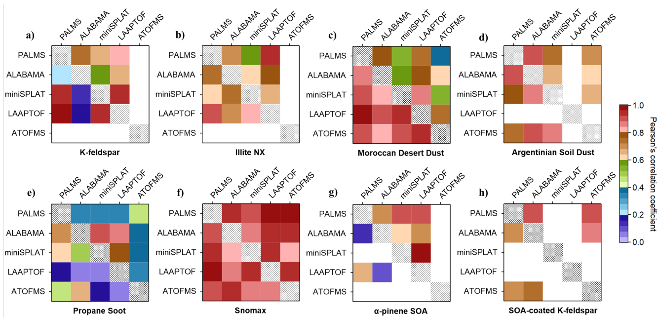
Figure 76: Correlation plots of average spectra of the different particle samples a) K-feldspar, b) Illite NX, c) Moroccan desert dust, d) Argentinian soil dust, e) propane soot, f) Snomax, g) \alpha -pinene SOA, and h) SOA-coated K-feldspar, analyzed by the five SPMs. Within each diagram correlation results for positive spectra are upper right and negative spectra are bottom left. White cubes denote cases where no data is available.
