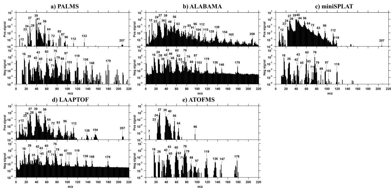
Figure 65: Normalized average mass spectra of Moroccan desert dust by a) PALMS, b) ALABAMA, c) miniSPLAT, d) LAAPTOF, and e) ATOFMS. The numbers of spectra averaged for each are 715 a), 353 b), 346 (c), 215 d), and 1447 e).
