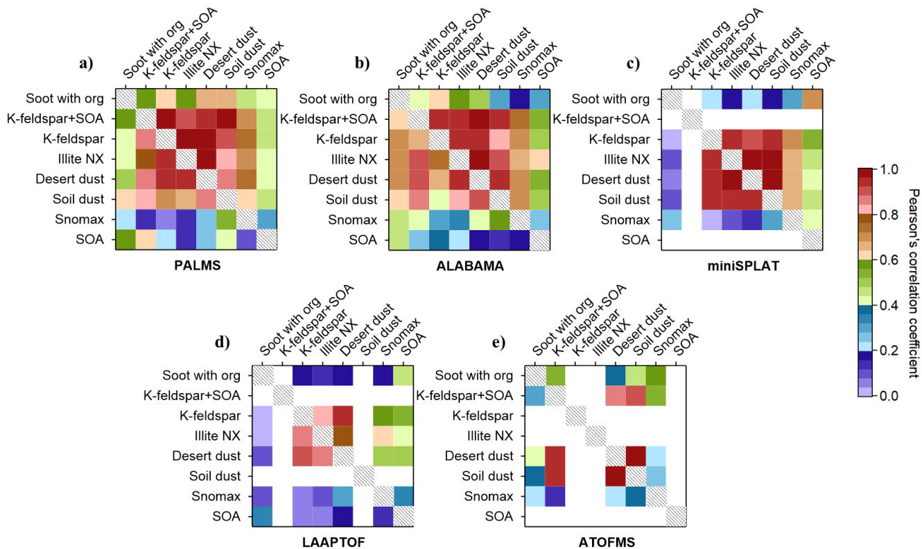
910 | Figure 87: Correlation plots of average spectra of different samples analyzed by a) PALMS, b) ALABAMA, c) miniSPLAT, d) LAAPTOF, and e) ATOFMS. Correlation results for positive spectra are upper right, while negative spectra are bottom left. Note that, the soot with organics and K-feldspar+SOA denote the propane soot and SOA-coated K-feldspar, respectively.
