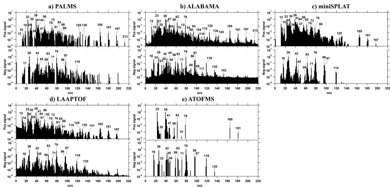
895 Figure 54: Normalized average mass spectra of Snomax, measured by a) PALMS, b) ALABAMA, c) miniSPLAT, d) LAAPTOF, and e) ATOFMS. The numbers of spectra averaged for each are 973 a), 1018 b), 2327 (c), 260 d), and 1071 e).
