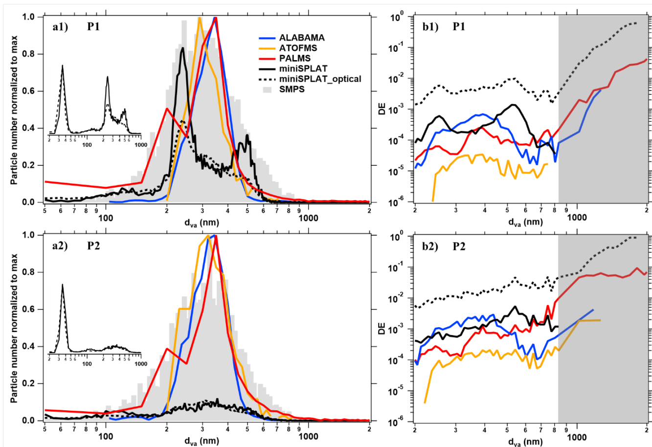
Figure 98: Particle size distribution and DE of PALMS (red), ALABAMA (blue), ATOFMS (orange), and miniSPLAT (black) during two different time periods (P1 and P2) of the blind experiments. For miniSPLAT, the full-size ranges measured during P1 and P2 are inserted in a1) and a2), respectively (note that the smallest size mode appears large, due to the lognormal mode in the X-axis). Note that the dashed black curves represent the DE of the whole size distribution measured by miniSPLAT, while in the solid black curve represent DE consistent with the other SPMSs (see text for details). d_m measured by SMPS (grey) was converted to d_{va} for comparison. The DE curves in the white and shaded areas are based on SMPS and APS results, respectively. f_m = 1.13 and f_{ca} = 1.06 , the number weighted values derived from \alpha -SOA and Argentinian soil dust (particle number ratio of 2:3), were used in these experiments. Note most of the soot particles were below the detection limit of SPMSs, with the exception of miniSPLAT (see text for details).
