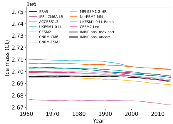
Figure 5. Ice mass over the historical period. All simulations are shown for medium sensitivity to outlet-glacier retreat forcing. The grey shadings represent the range of observed mass loss data from Shepherd et al. (2020), with light grey shading indicating the assumption of maximal error correlation and dark grey shading indicating uncorrelated errors. The IMBIE treatment of errors involves two approaches: maximal error correlation assumes that errors across different datasets are fully correlated, leading to a wider uncertainty range (light grey shading). In contrast, uncorrelated errors assume no correlation between errors in different datasets, resulting in a narrower uncertainty range (dark grey shading).
