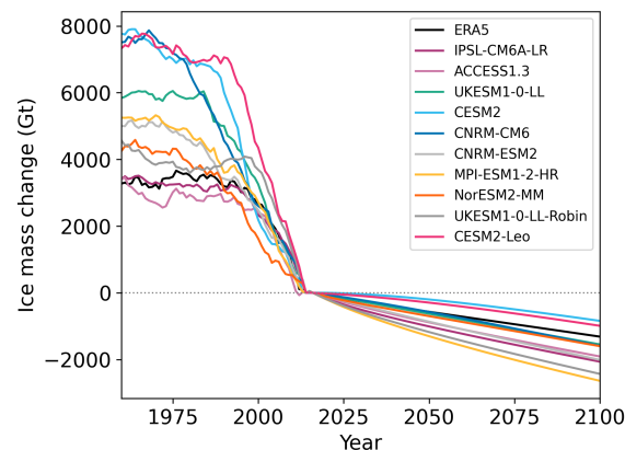
Figure 7. Mass loss (in Gt) of different ice sheet configurations over the historical period and subsequent control projections with forcing set to the mean of the reference period 1960–1989.
