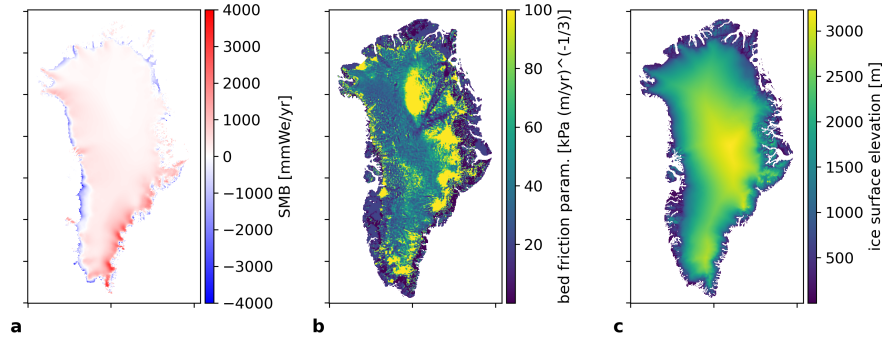
Figure 2. SMB (a), bed friction parameter (b) and ice surface elevation (c) at the end of the initialization of ERA5-init.
