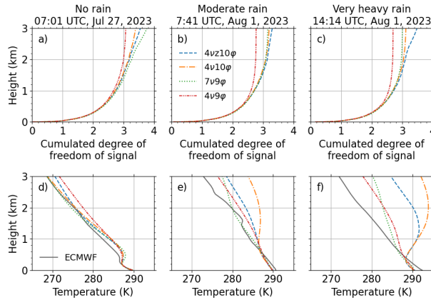
Figure 5. The cumulated degrees of freedom of signal and temperature profiles T-profiles for no rain (a, d) conditions on Jul 27, 2023, moderate rain (b, e) and heavy rain (c, f) conditions on Aug 1, 2023.
