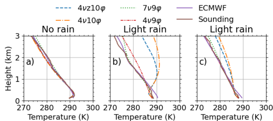
Figure 8. Panels a, b, and c show a comparison of three retrieved temperature profiles-T-profiles obtained from the four different retrievals with radio-soundings launched at MOL-RAO on Aug 26, 2020, at 4:45 (a), 10:45 (b), and 22:45 UTC (c) and ECMWF model output from 5, 11, and 23 UTC.
