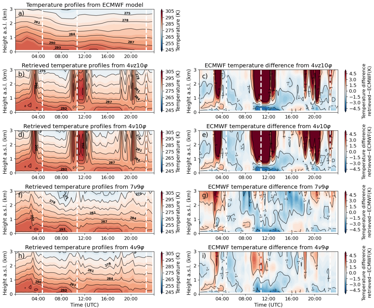
Figure 7. Height-time series of temperature profiles-T-profiles from ECMWF model (a) and temperature profiles-T-profiles based on different retrieval algorithms (b, d, f, h) and associated temperature difference to ECMWF model (c, e, g, i) in Lindenberg (Germany) on Aug 26, 2020. The radiosonde launch times are indicated by white dashed lines.
