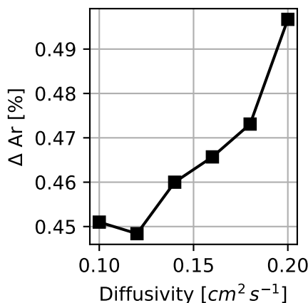
Figure 9. Simulated argon oversaturation as a function of explicit background diffusivity. Each value corresponds to a Coarse simulation with respective diffusivity for temperature, salinity and Ar. The argon oversaturation is calculated as averaged horizontally over the high-resolution model domain ( 30^\circ W - 15^\circ W and 17^\circ N - 24^\circ N ) and vertically over 100 to 400 m depth. For reference, simulation High features 0.43% (Table 2).
