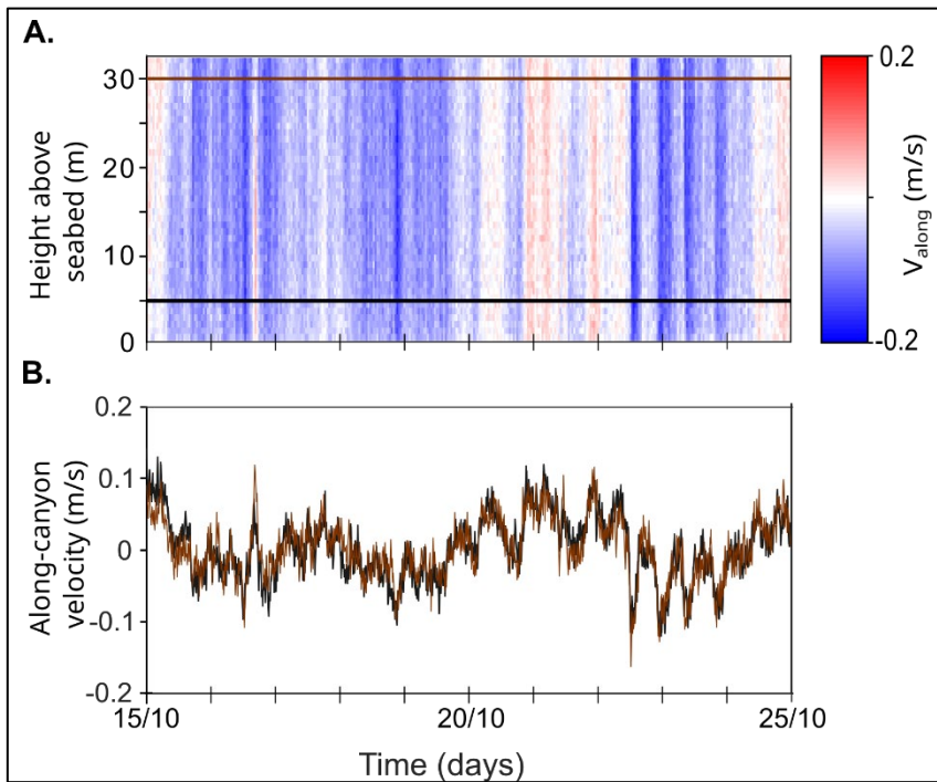
605 Figure A2: Velocity along canyon ( V_{\text{along}} ) and frequency analysis for the period 15 th to 25 th October 2019 (see Fig. 2A for context). A. Time series of V_{\text{along}} between 15 th October and 25 th October 2019. The brown and black horizontal lines indicate the locations of the arrays displayed in B. B. V_{\text{along}} speeds at 5 and 30 m above canyon floor.
