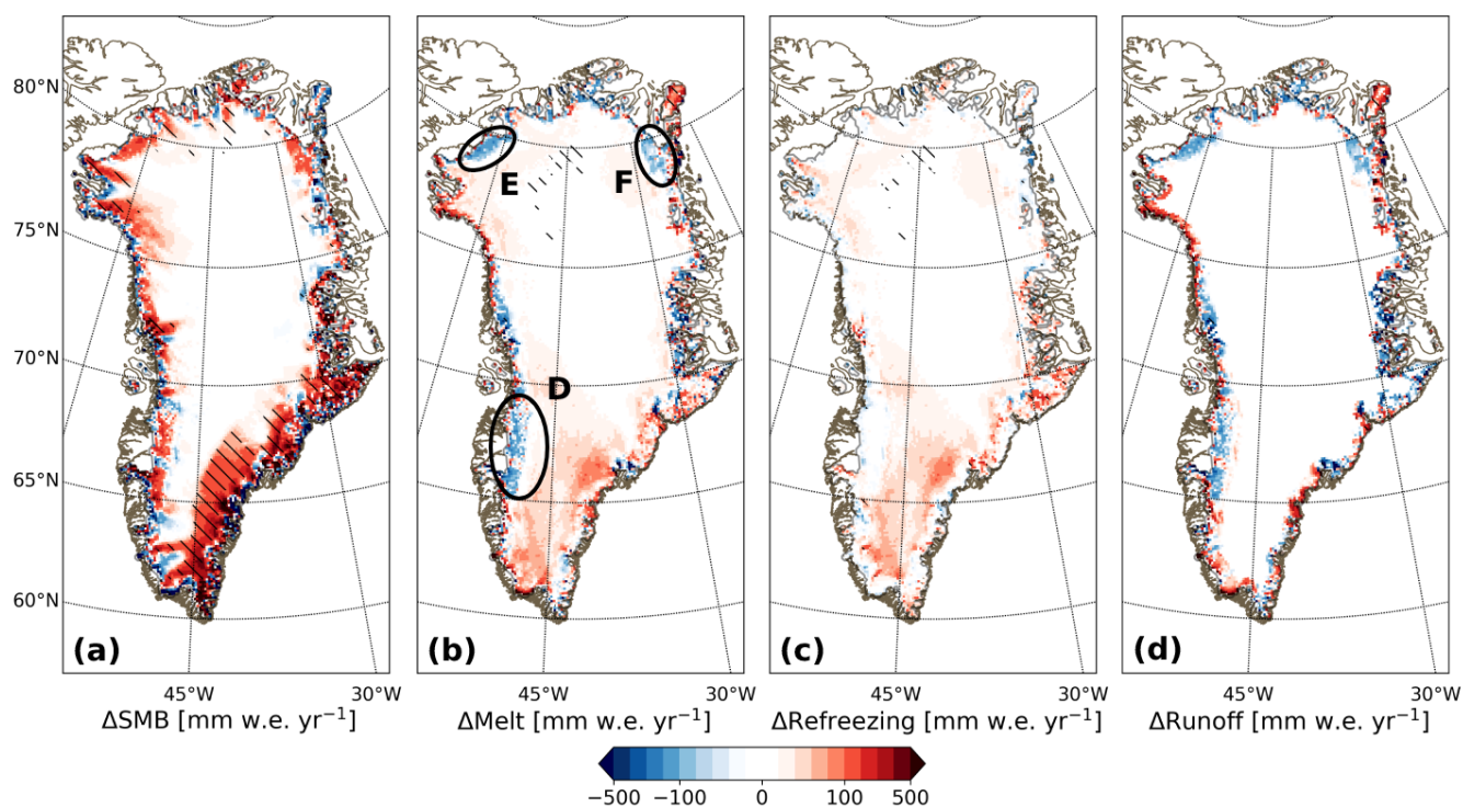
Figure 5. Average (2006-2015) difference (R24 - R23p3) for (a) SMB, (b) melt, (c) refreezing and (d) runoff in mm w.e. yr -1 . The same color scale as in Fig. 3b is applied. Differences larger than inter-annual variability are hatched. Regions D , E and F are discussed in the text.
