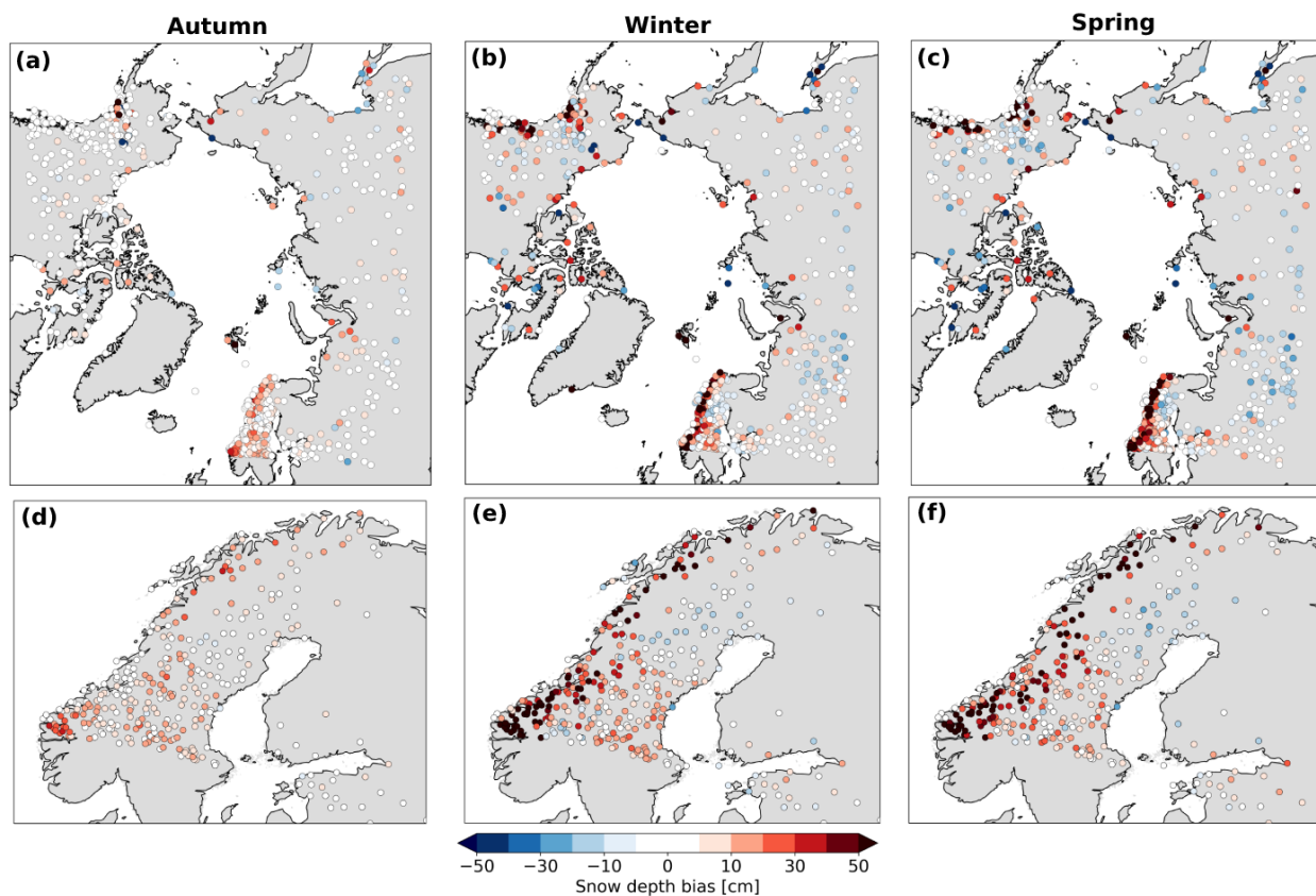
Figure 10. Daily snow depth bias of R24 with respect to in-situ observations for 2002-2003 for autumn (a), winter (b) and spring (c), with stepsizes of 10 and 5 cm between -50 to -10 and 10 to 50, and -10 to 10 cm, respectively. Scandinavia is shown separately in (d)-(f). Red illustrates an overestimated snow depth in R24. Data points in the boundary relaxation zone (24 grid cells wide) are excluded from the analysis.
