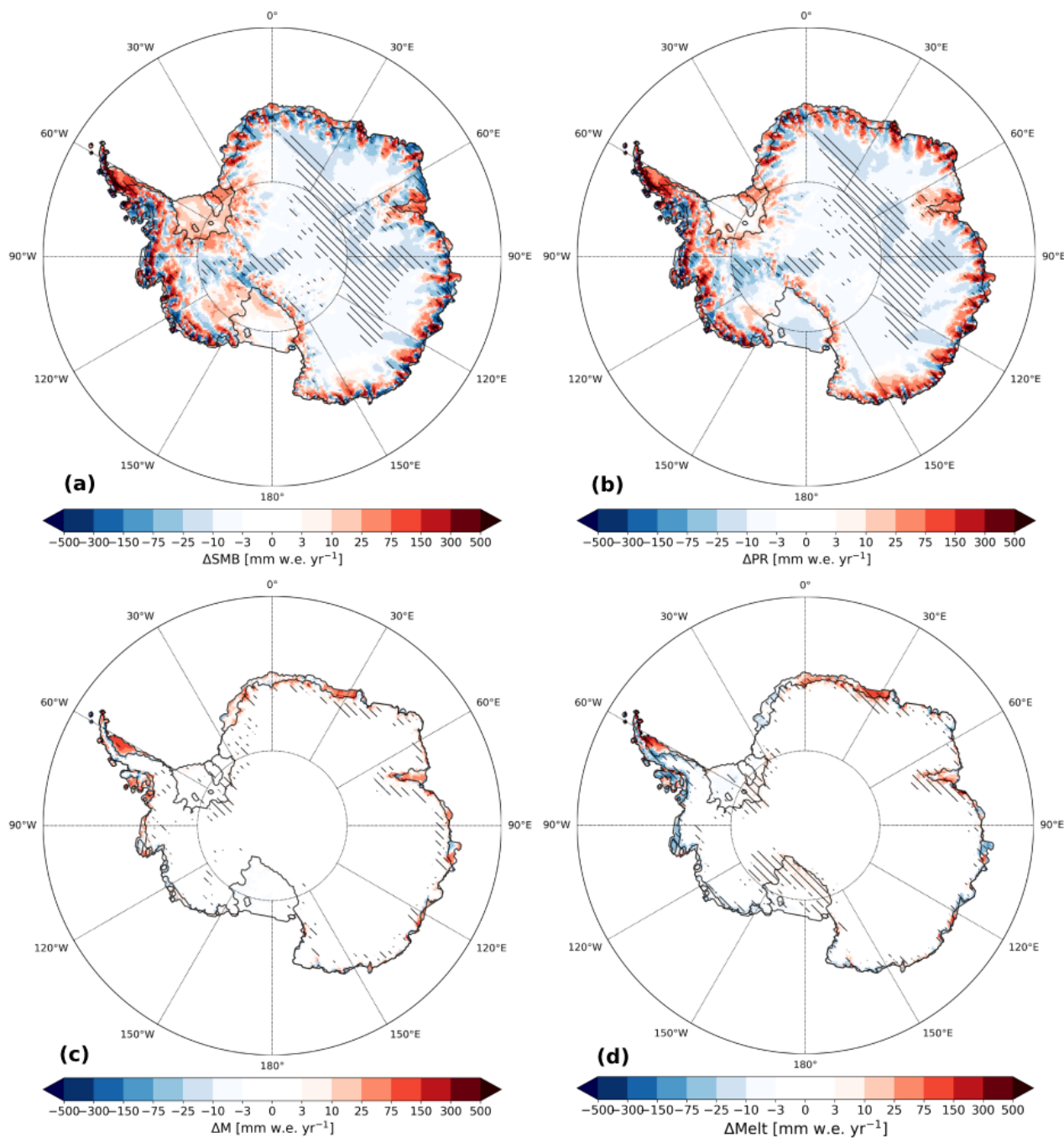
Figure 8. Average (2006-2015) difference (R24 - R23p3) for (a) SMB, (b) precipitation and (c) melt. (d) Annual-average melt difference with QSCAT (R24 - QSCAT) for 2007-2009. Differences larger than inter-annual variability are hatched.
