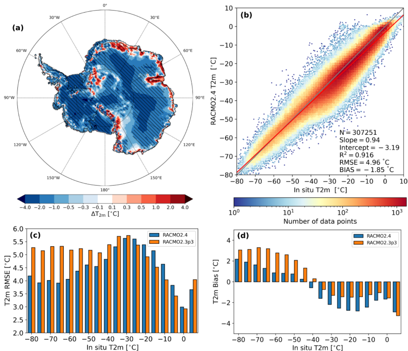
Figure 9. (a) Annual-average T2m difference (R24 - R23p3) for 2006-2015. Differences larger than inter-annual variability are hatched. (b) Daily-average T2m for R24 with respect to AntAWS measurements (locations are shown in Fig. 1b). The 1-on-1 line is shown in gray. Bias, root-mean-square error (RMSE), determination coefficient ( R^2 ), intercept and slope of orthogonal total least squares regression, and number of points (N) are also shown. (c) RMSE and (d) bias for R24 and R23p3 with respect to AntAWS for T2m, with 5 °C bins.
