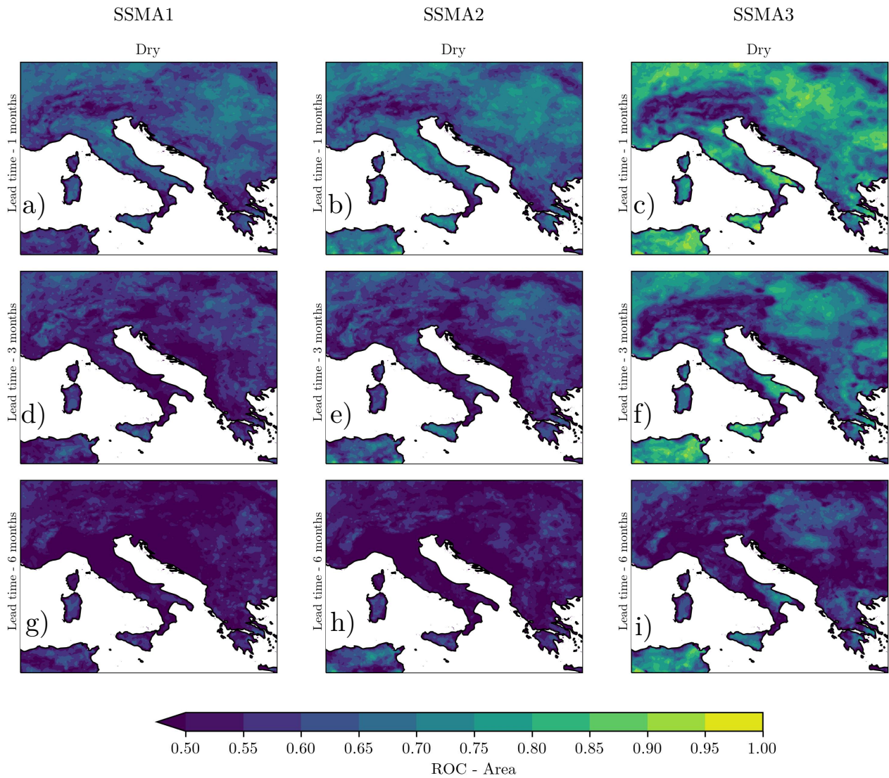
Figure 10. Area under the ROC curve averaged over all dry events during 2001-2021 for: (a,d,g) soil layer 1 (7 cm) SSMA1; (b,e,h) soil layer 2 (28 cm) SSMA2; (c,f,i) soil layer 3 (100 cm) SSMA3. Different rows concern different lead-times.
