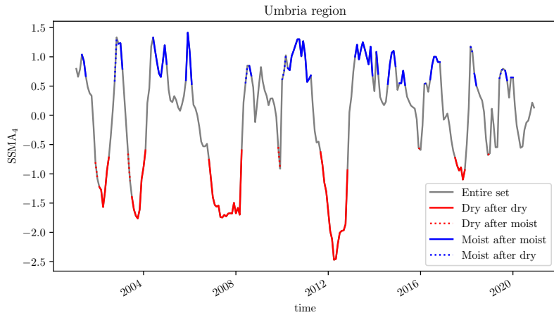
Figure 12. Example of event selection based on soil moisture pre-condition over the Umbria reference point for ERA5-LAND SSMA in the deepest soil layer 4 (289 cm). Dry periods are considered as those with SSMA < -0.5 , while wet periods are those with SSMA > 0.5 . A period is considered to happen after a dry period when the SSMA evaluated three months earlier is negative ( SSMA < 0 ), while a period is considered to happen after a wet period when the SSMA evaluated three months earlier is positive ( SSMA > 0 ). The result of such a selection is reported with the following lines: entire time series (gray solid line), dry period after a dry period (red solid line), dry period after a wet period (red dotted line), wet period after a dry period (blue dotted line), wet period after a wet period (blue solid line).
