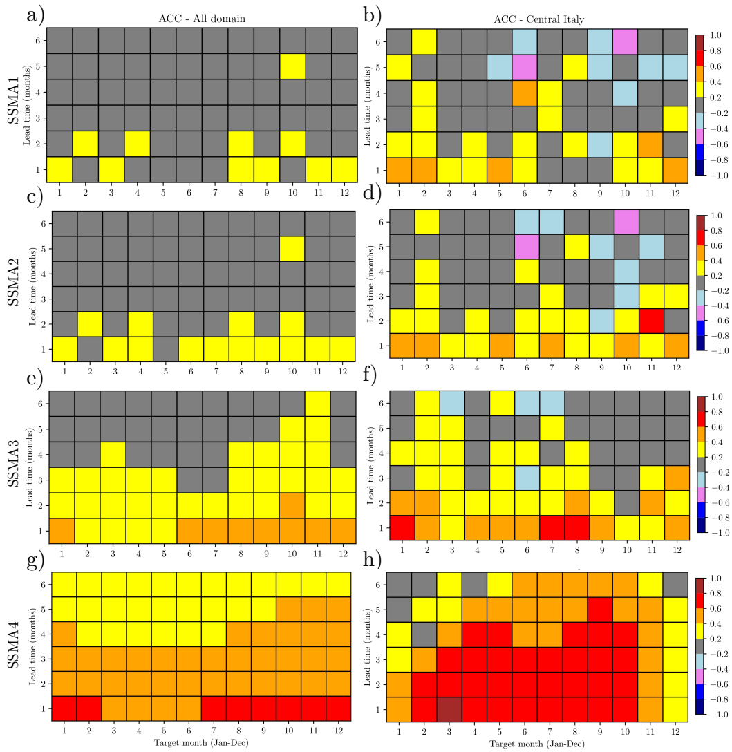
Figure 9. Area averaged Anomaly Correlation Coefficient (ACC) for each target month (x axis) and for different lead-times (y axis). Average values are computed over the whole domain (a,c,e,g) and Central Italy (b,d,f,h, black squared areas reported in Figure 1a). Rows show different soil layers: top layer (SSMA1, 7 cm depth), second layer (SSMA2, 28 cm depth), third layer (SSMA3, 100 cm depth), and bottom layer (SSMA4, 289 cm depth).
