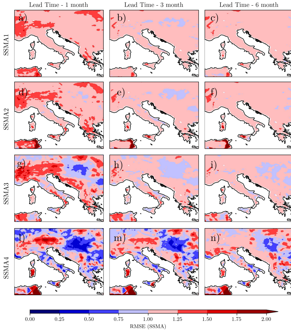
Figure 7. RMSE of Standardized Soil Moisture Anomalies (SSMA) averaged over the whole analyzed period (2001-2021). Rows show different soil layer: (a,b,c) soil layer 1 (7 cm); (d,e,f) soil layer 2 (28 cm); (g,h,i) soil layer 3 (100 cm); (l,m,n) soil layer 4 (289 cm). Columns show the same statistics for the forecast values at different forecast lead-times (1, 3, and 6 months).
