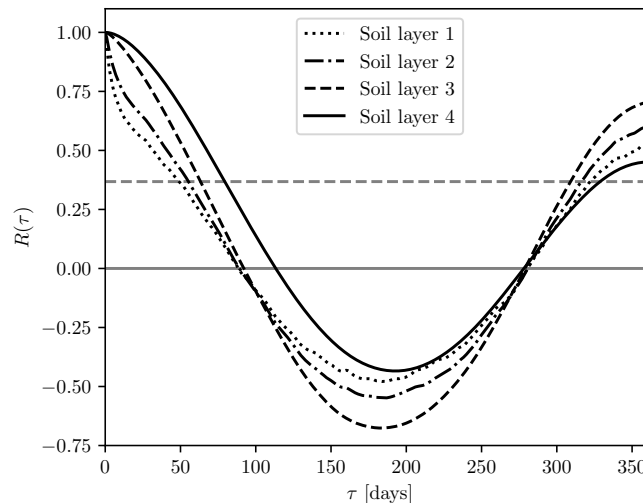
Figure 3. Memory time scale over Umbria region for the different soil layers: soil layer 1 (dotted line), soil layer 2 (dashed-dotted line), soil layer 3 (dashed line), soil layer 4 (solid line). The temporal correlation refers to the time series shown in Figure 2. The dashed gray line represents the threshold e^{-1} and the corresponding e-folding time (the time when correlation is lower than this threshold) represents the memory time scale of each soil layer.
