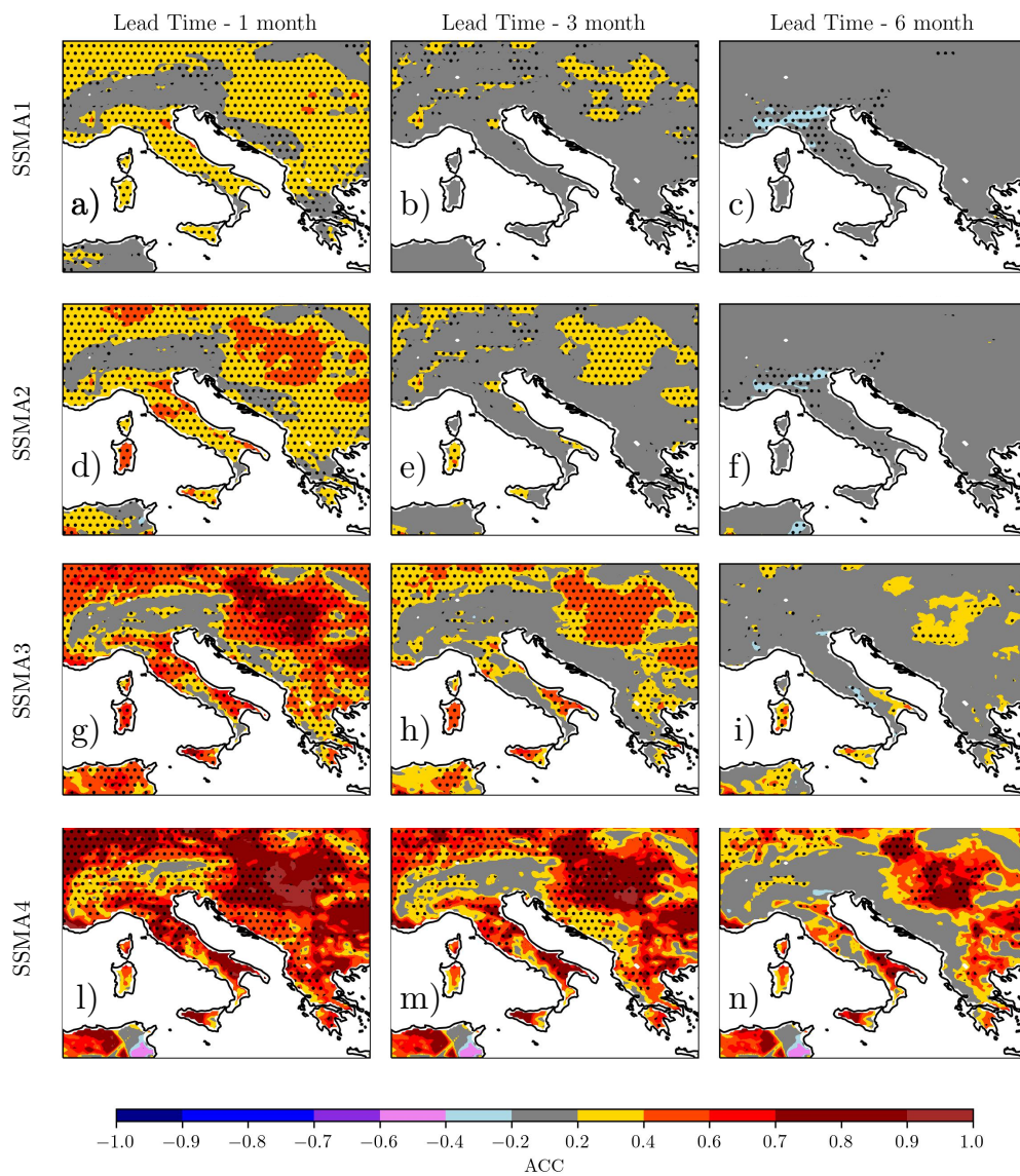
Figure 8. Anomaly Correlation Coefficient (ACC) of Standardized Soil Moisture Anomalies (SSMA) averaged over the whole analyzed period (2001-2021). Rows show different soil layer: (a,b,c) soil layer 1 (7 cm); (d,e,f) soil layer 2 (28 cm); (g,h,i) soil layer 3 (100 cm); (l,m,n) soil layer 4 (289 cm). Columns show the same statistics at different forecast lead-times (1, 3 and 6 months). Significant correlation ( p -value < 0.05) are marked with black dots.
