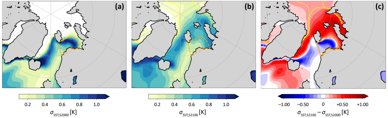
Figure 7. SST standard deviation (in K) in (a) S2000 ( \sigma_{SST,S2000} ) and (b) S2100 ( \sigma_{SST,S2100} ). Panel (c) shows the difference between S2000 and S2100 ( \sigma_{SST,S2100} - \sigma_{SST,S2000} ). The climatological sea ice edge is shown as solid yellow line for S2000 and as dashed yellow line for S2100. Region BS is marked with orange line.
