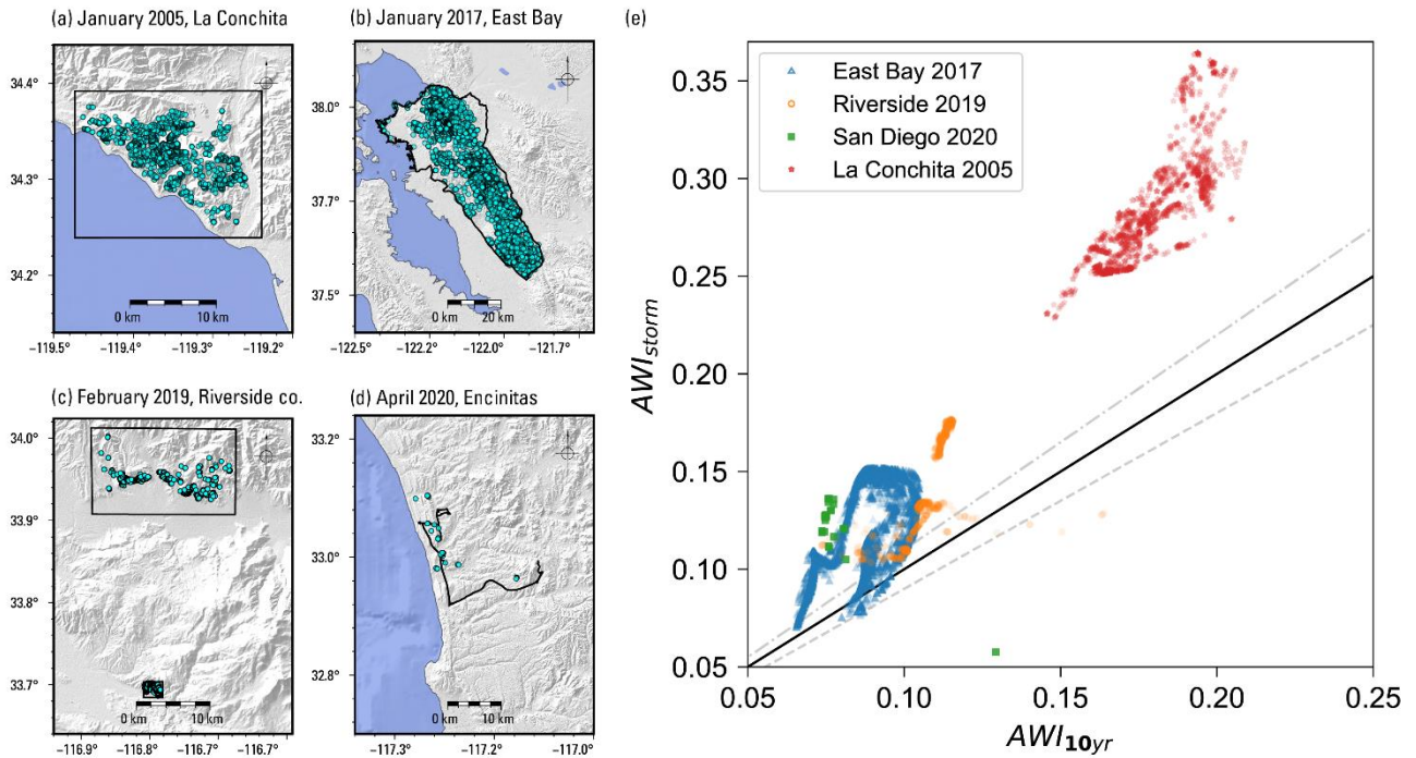
355 Figure 3. Landslide inventories (a-d) used to estimate a reasonable antecedent water index ( AWI ) recurrence threshold above which most landslides occurred. Black boxes and polygon in panels (a)-(c) represent the landslide mapping bounds for each event, and black line in panel (d) represents the GPS tracks from CGS field mapping campaign. Panel (e) shows a plot of peak AWI modelled during the storm windows interpolated to each landslide point (y-axis) against the 10-year recurrence AWI at each point (x-axis). A constant threshold across regions would plot as a horizontal line. Over 97% of the mapped landslides plot above their 360 10-year recurrence value (the 1:1 line). Dashed lines are the 0.9:1 and 1.1:1 lines. Shaded relief for (a)-(d) derived from NASA SRTM 30 m DEM (NASA, 2013).
