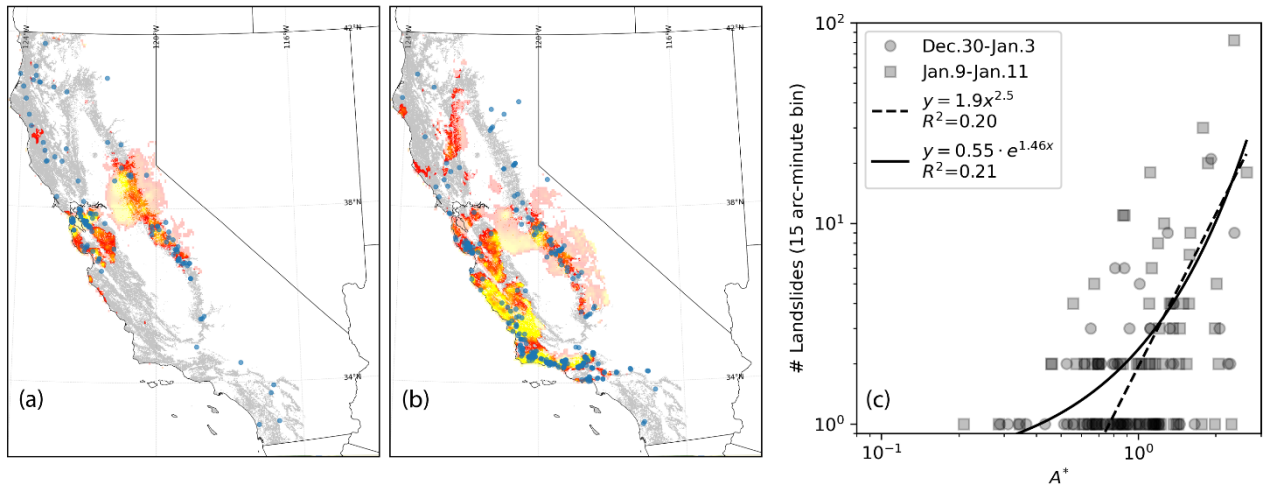
Fig. 10. Maps showing distributions of A^* maxima and reported landslides during two periods of the December 2022 - January 2023 atmospheric river sequence: (a) 30 December – 03 January which strongly impacted the San Francisco Bay area; and (b) 09 January – 11 January, which strongly impacted the central coast and southern California. Yellow symbols are landslides from each time period from the California Geological Survey Reported Landslides. Panel (c) shows a plot relating a grid of landslide point density (y-axis) to A^* maxima for each respective period in the storm sequence. Although a number of isolated slides show low values of A^* , as A^* approaches 1 landslide density begins to rise rapidly. This highlights the efficacy of the method for identifying zones of widespread landsliding rather than locally isolated events. Shaded relief in (a) and (b) from NASA SRTM 30 m DEM (NASA, 2013).
