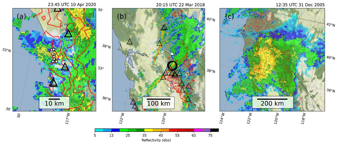
530 Figure 9. Maps showing examples of a range of spatial scales of precipitation influencing landslide-inducing rainfall distribution in California. Radar reflectivity values are shown as colored pixels, and associated A^* > 1 values for each storm are shown as red contours. (a) Mesoscale features such as isolated thunderstorms produced very high intensity rainfall and led to localized landslide hotspots in the April 2020 storm in southern California (Table 1; black circles). (b) Narrow cold frontal rainbands (NCFR), on the order of a few km wide and tens of km long, are another mesoscale feature that can produce high-intensity rainfall, leading to
