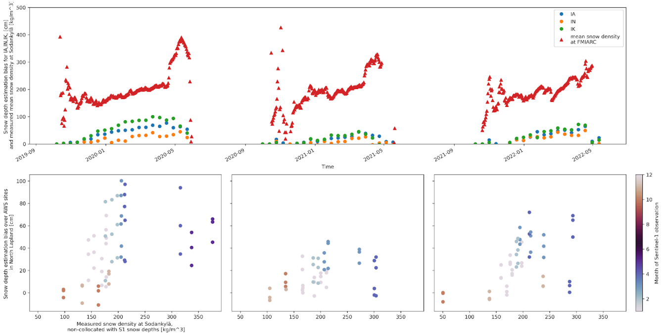
3 Figure S1: Bias evolution of the snow depth as a function of the days of the year.
