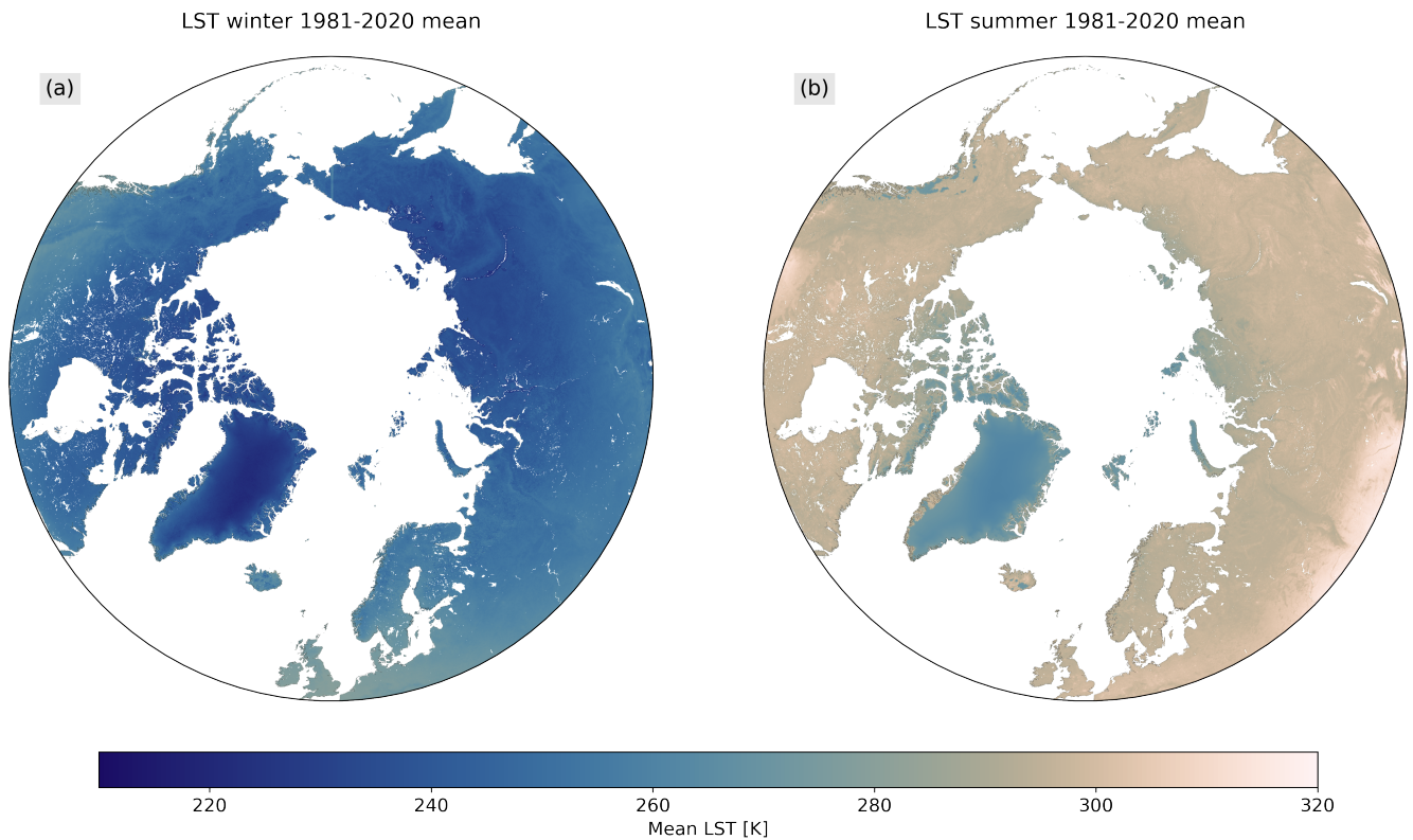
Figure 12. Mean LST (1981-2020) for (a) winter and (b) summer.
