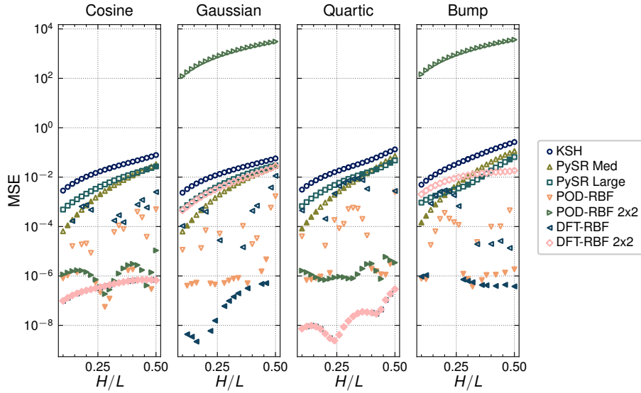
Figure 12. MSE for all shear stress perturbation models grouped by profile. The PODF-RBF 2x2 and DFT-RBF 2x2 results refer to the two profile trained models. Filled marks indicate cases used for training where the reported MSE represents the reconstruction error and empty marks represent test cases where the reported MSE represents the prediction error compared to the CFD results.
